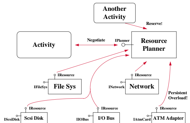
Figure 3-4: Resource Negotiation
