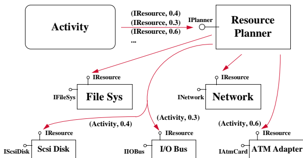
Figure 3-3: Resource Reservation
