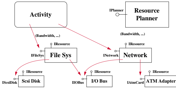
Figure 3-2: Resource Queries
