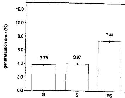
Figure 4: Percentage of generalisation errors made by IGTREE on the GS task, in terms of the percentage incorrectly classified test instances as well as on phonemes and stress assignments computed separately.
