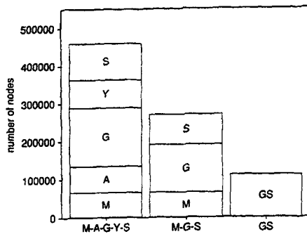
Figure 5: Average numbers of nodes in the decision trees generated by IGTREE for the M-A-G-Y-S, M-G-S, and GS systems. Compartments indicate the numbers of nodes needed for the trees of the subtasks specified by their labels.
