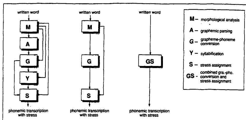
Figure 1: Architectures of the three investigated word-pronunciation systems. Left: M-A-G-Y-S; middle: M-G-S; right: GS. Rectangular boxes represent modules; the letter in the box corresponds to the subtask as listed in the legenda (far right). Arrows depict data flows from the raw input or a module, to a module or the output.
