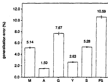
Figure 2: Generalisation errors on the M-A-G-Y-S system in terms of the percentage of incorrectly classified test instances by IGTREE on the five subtasks M, A, G, Y, and S, and on phonemes and stress markers jointly (PS).
