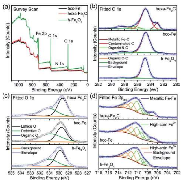
Fig. 2 (a–d) Binding and fitted X-ray photoelectron spectra (XPS) of hexa-Fe 2 C, bcc-Fe and Fe 3 O 4 NPs. (a) Survey scan. (b) C 1s region. (c) O 1s region and (d) Fe 2p 3/2 region fitted using Gupta–Sen multiplets.
