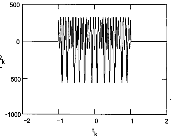
1a. Channel 2 Deconvolver ( v_2 ).
