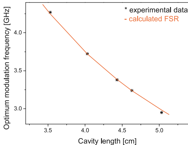
Fig. 3 The effect of the cavity length on the modulation response. For every cavity length we searched for the strongest modulation response. The experimental data are fitted to the theoretical formula FSR = c/2L_{\text{eff}} . The error bars are too small to be shown on this scale. In this work we focus on this optimal configuration in which the modulation frequency equals the FSR
