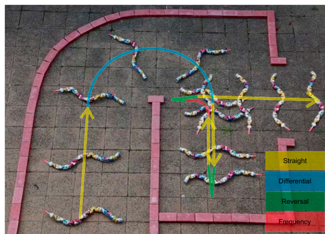
Fig. 6. Images from Movie S6 showing the sidewinder robot moving through a trackway using three turn types (labeled) and straight-line sidewinding. The size of the test course is 3 × 3 m 2 and the robot completed the course in 48 s.
