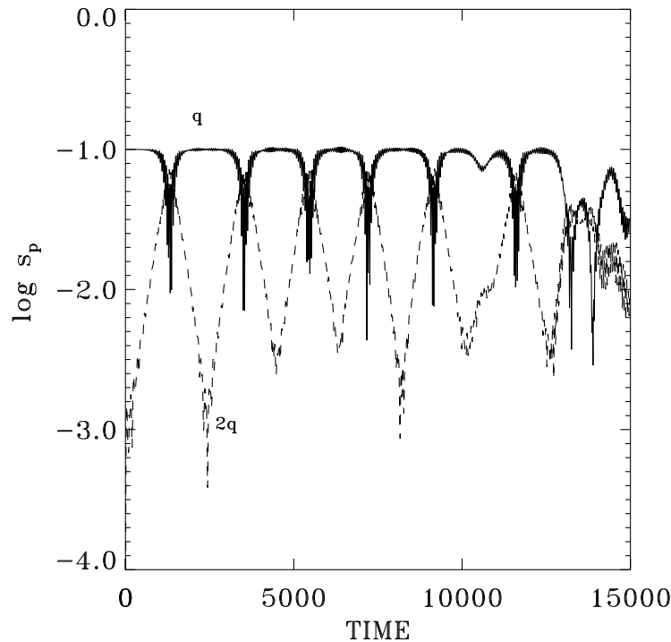
Figure 5. Recurrence. Evolution of the amplitude of the Fourier transform for wave numbers q and 2q versus time ( q = 0.491 ). The parameters are \alpha = 15 , K = 1 , \phi_0 = 0.1 and \omega_0^2 = 100 . A logarithmic scale is used for the ordinate.
