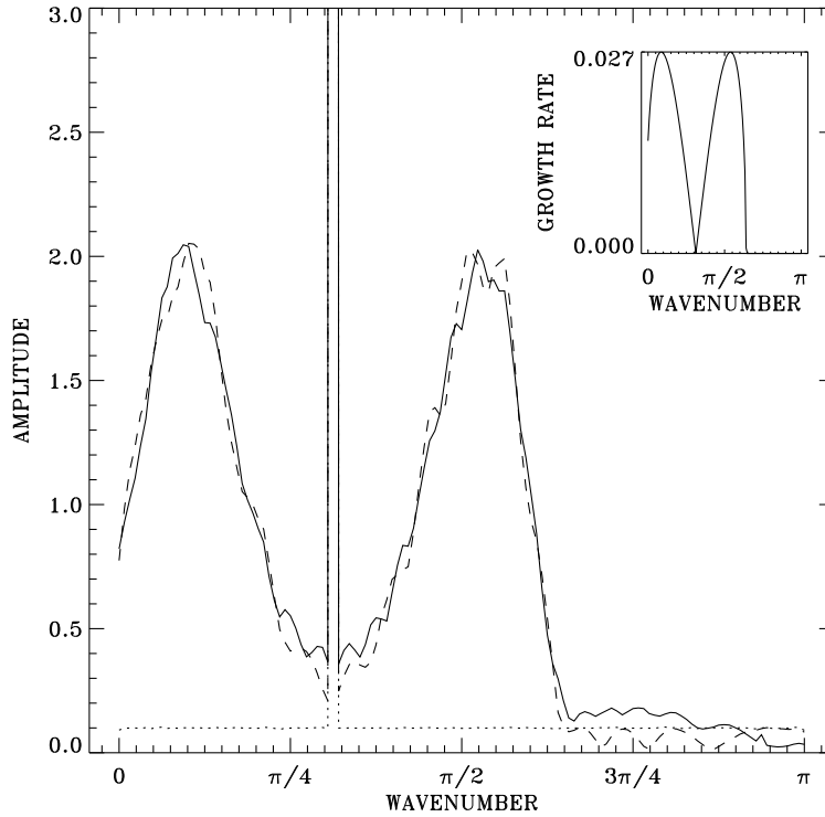
Figure 6. Noise. Amplitude of the Fourier transform of the positions versus the wavenumbers. The solid curve corresponds to the numerical results obtained at t = 150 by averaging 1000 simulations, the dotted curve to the initial condition and the broken curve to the analytical expression (see text). The inset presents the growth rate expression versus the wavenumber. Parameters are \beta = 0.5 , K = 2 , \phi_0 = 0.6 , \omega_0^2 = 100 and t_0 = 100 . The amplitude of the gaussian noise is 0.01 and its variance is 1.
