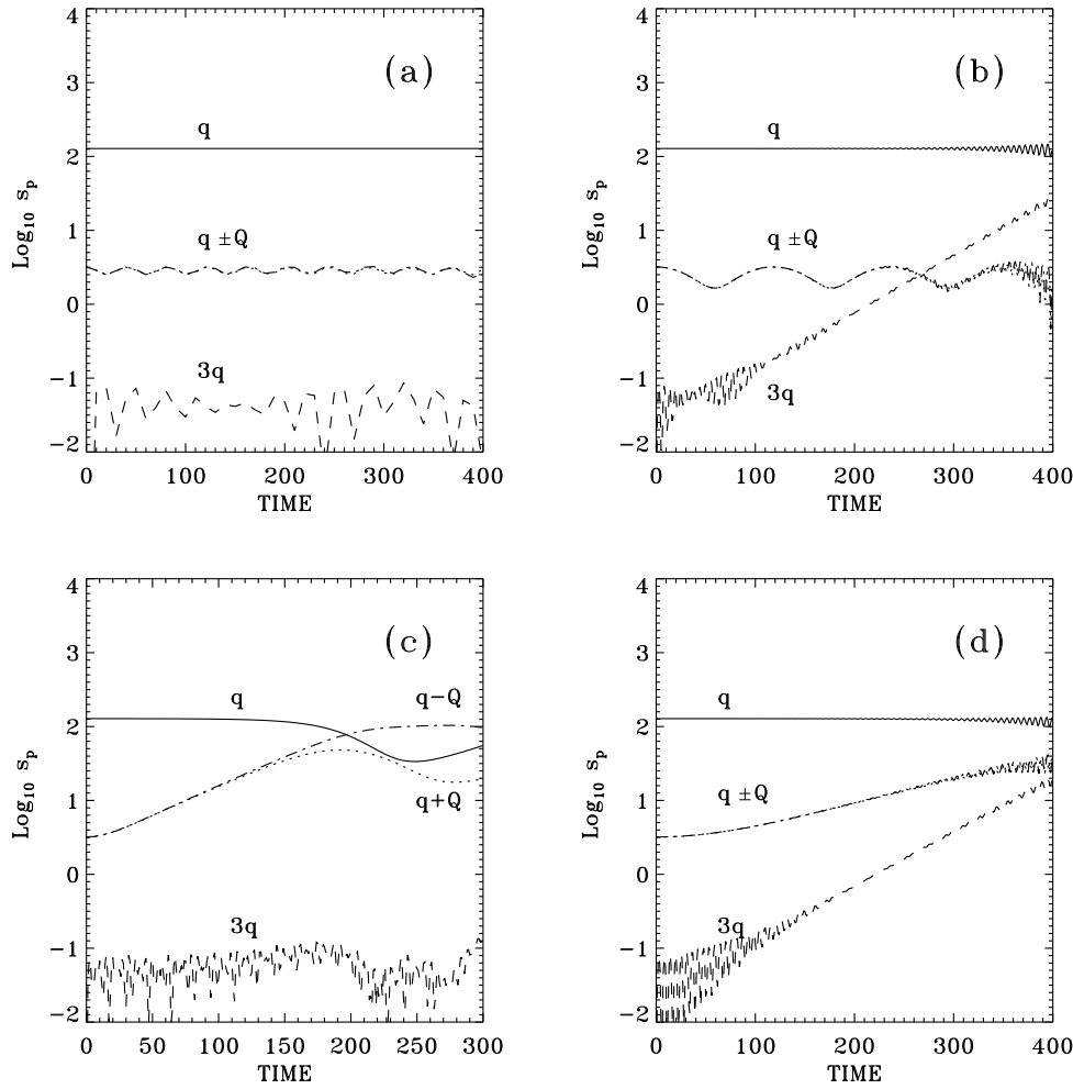
Figure 3. Evolution of the amplitude of the Fourier transform for different wavenumbers. The solid line corresponds to the initial frequency q , the dotted line to (q + Q) , the dash-dotted line to (q - Q) and the dashed line to 3q . The frequencies q and Q are determined from p = 80 and P = 200 for (a), p = 30 and P = 80 for (b), p = 80 and P = 60 for (c), p = 30 and P = 110 for (d). The parameters are \beta = 0.5 , K = 1 , \phi_0 = 0.5 and \omega_0^2 = 100 . A logarithmic scale is used for the ordinate.
