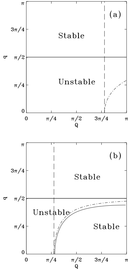
Figure 1. Stability curve. Figure (a) presents a case where \phi_{0_c} < \phi_0 while (b) depicts the opposite case \phi_{0_c} > \phi_0 . The solid curve corresponds to the discrete condition (9), the dot-dashed curve to the semi-discrete and the dashed curve to the continuum limit. The words stable and unstable correspond to the discrete condition. The parameters are \omega_0 = 10 , K = 1 , \beta = 1 and \phi_0 = 1 for figure (a) and \omega_0 = 10 , K = 1 , \beta = 0.5 and \phi_0 = 0.5 for (b).
