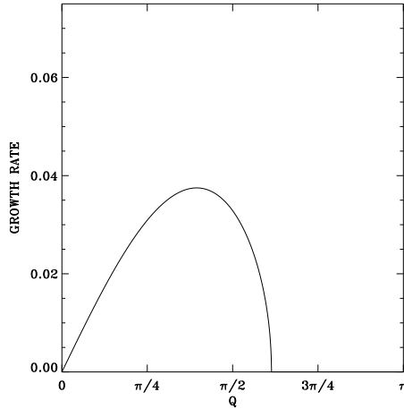
Figure 2. Growth rate versus the wavenumber of the perturbation. This case corresponds to the parameters \omega_0 = 10 , K = 1 , \beta = 1 and \phi_0 = 1 and q = 5\pi/8 .
