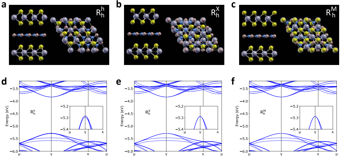
Extended Data Figure 3 — Band structure of R-stacked \text{MoSe}_2/\text{hBN}/\text{MoSe}_2 heterostructure obtained from density functional theory (DFT) calculation. a to c show the side and top view of the supercell used for the calculation. d, e and f show the calculated band structure of R-stacked \text{MoSe}_2/\text{hBN}/\text{MoSe}_2 for R_h^h , R_h^X and R_h^M lattice displacement, respectively. The insets show the magnified plot of the valence bands around \gamma point.
