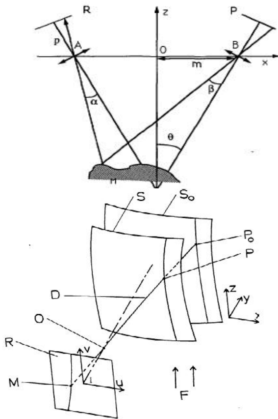
Figure 1: Experimental device of the geometry method
