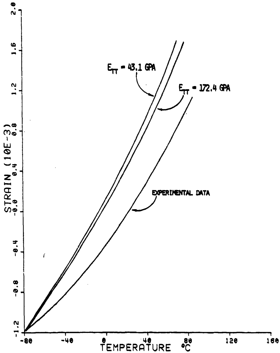
Figure 80. Moisture Conditioned Transverse Thermal Expansion Sensitivity to Young's Modulus of the Fiber for S2 Glass/3901-6 Glass/Epoxy (Base Value E_{TT} = 86.2 \text{ GPa} )
