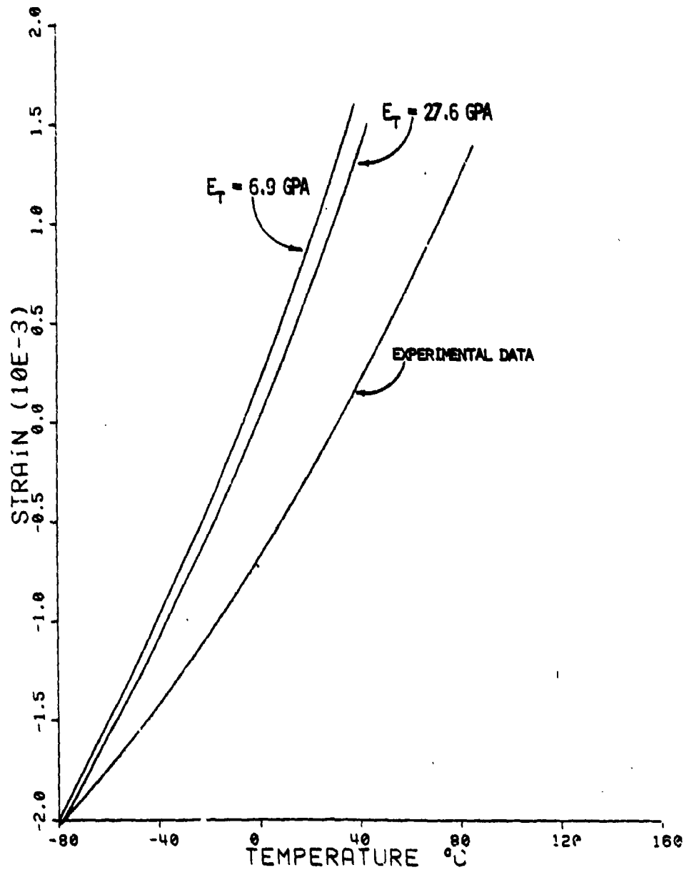
Figure 68. Moisture Conditioned Transverse Thermal Expansion Sensitivity to Transverse Young's Modulus of the Fiber for AS/3501-6 Graphite/Epoxy (Base Value E_T = 13.8 GPa)
