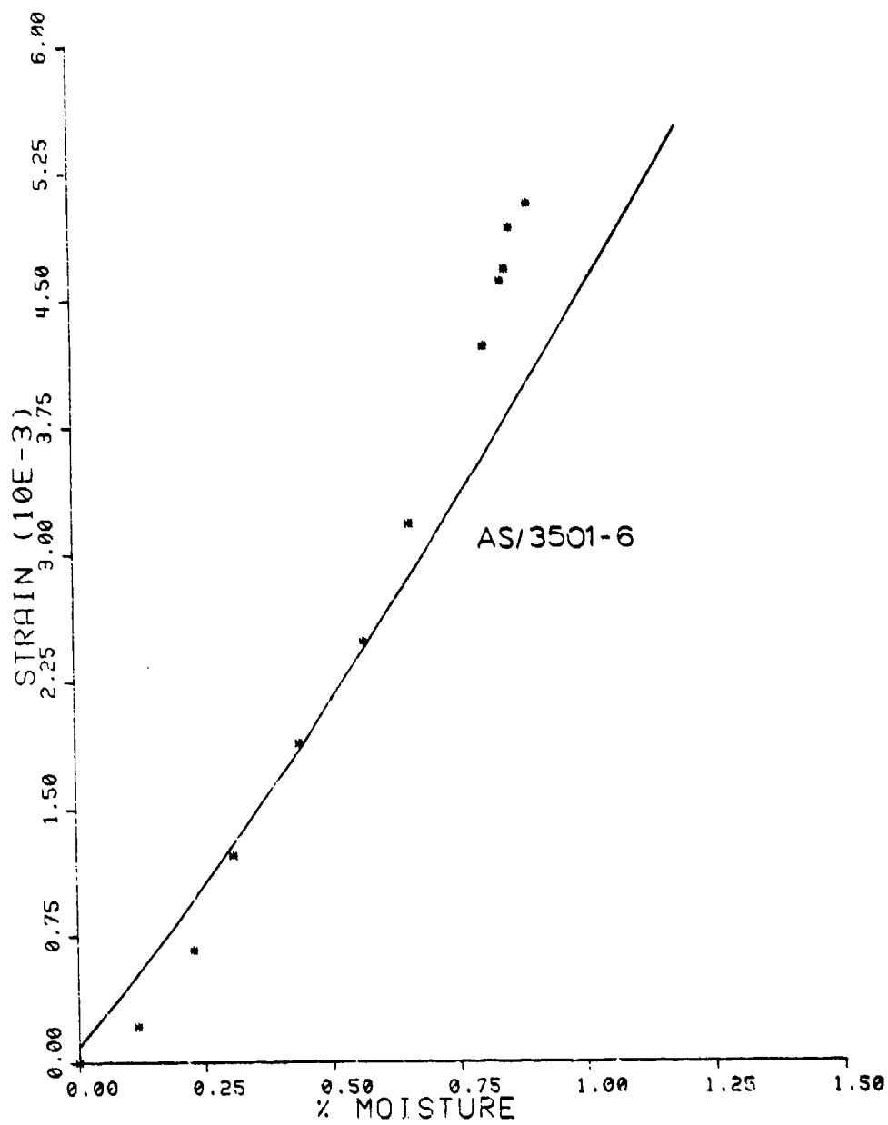
Figure D8. Results of Test 1, Station J, 10 days @ 98% RH, 65.5°C (150°F)
