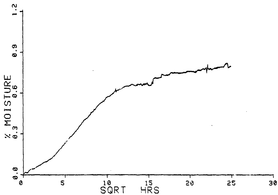
Figure 25. Typical Diffusivity Curve for S2 Glass/3501-6 from NPLDT RH = 98%, Temperature = 65.5°C (150°F), Thickness = 0.86 mm (0.034 in)
