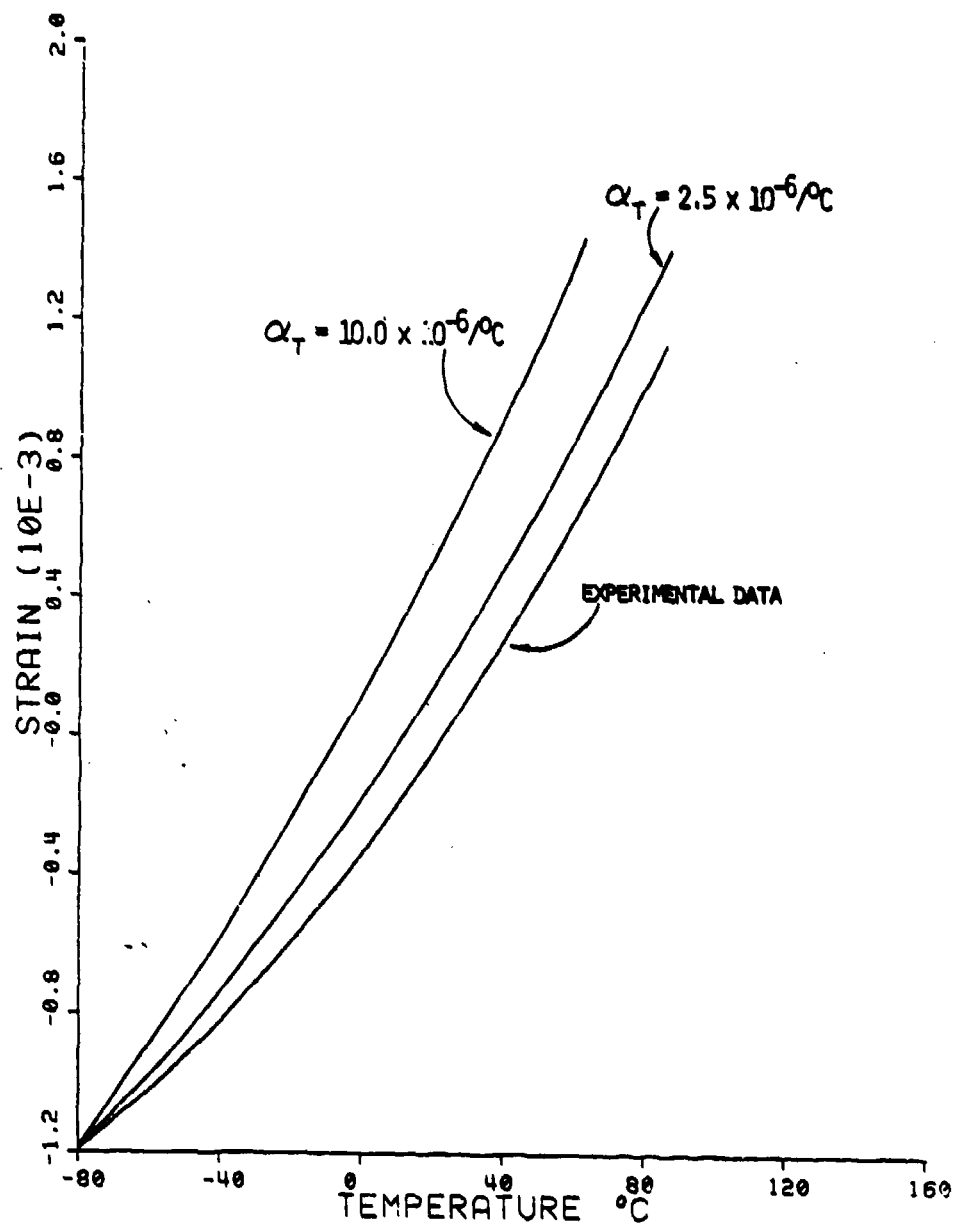
Figure 81. Moisture Conditioned Transverse Thermal Expansion Sensitivity to Transverse Thermal Expansion of the Fiber for S2 Glass/3501-6 Glass/Epoxy (Base Value \alpha_T = 5.0 \times 10^{-6}/^{\circ}\text{C} )
