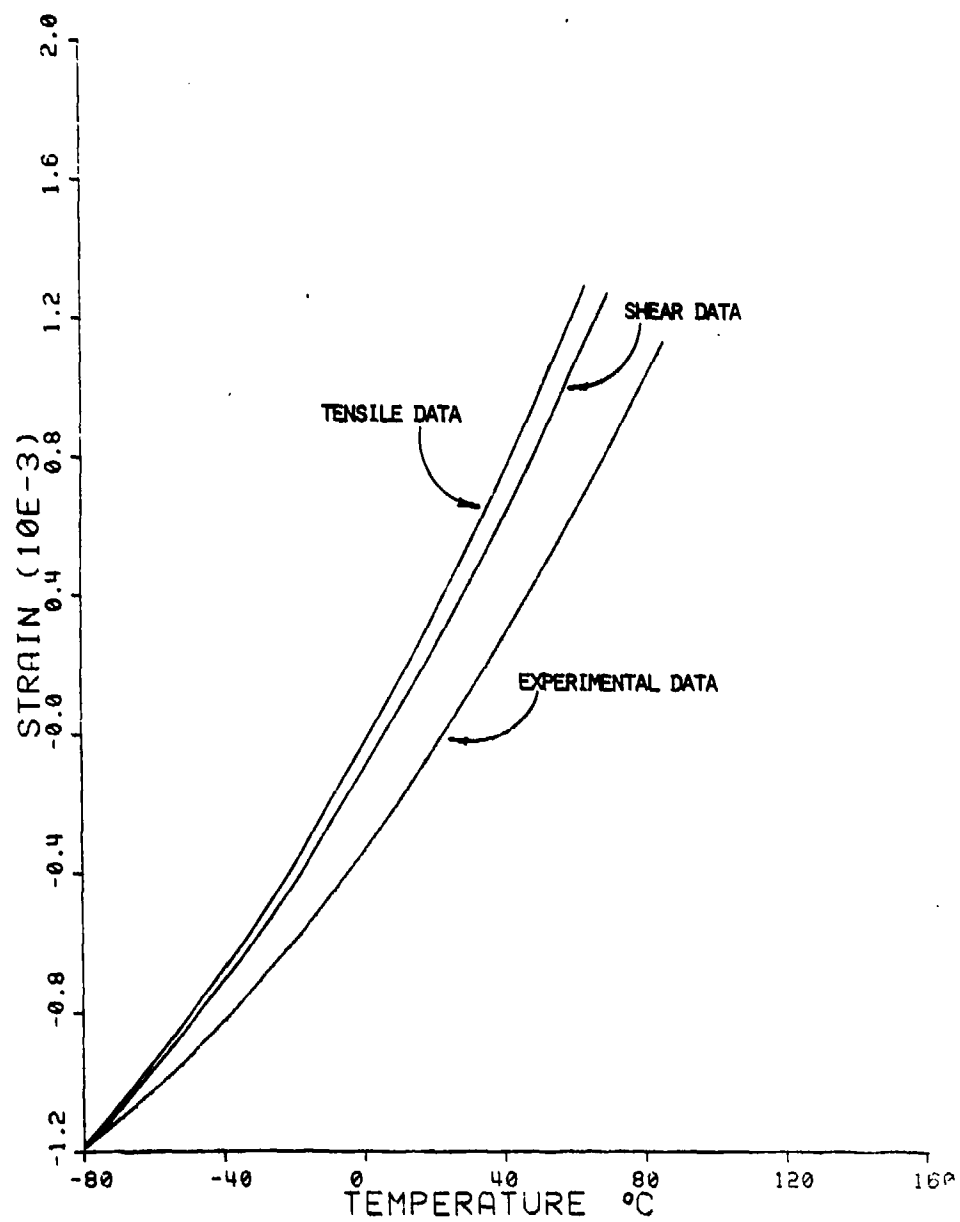
Figure 76. Moisture Conditioned Micromechanics Predictions of Thermal Expansion for 52 Glass/3501-6 Glass/Epoxy in the Composite Transverse Direction
