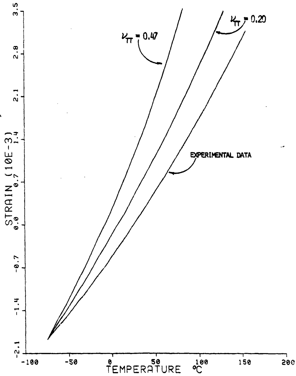
Figure 59. Unconditioned Transverse Thermal Expansion Sensitivity to Poisson's Ratio of the Matrix for AS/3501-6 Graphite/Epoxy (Base Value of Matrix \nu_{TT} = 0.34 )
