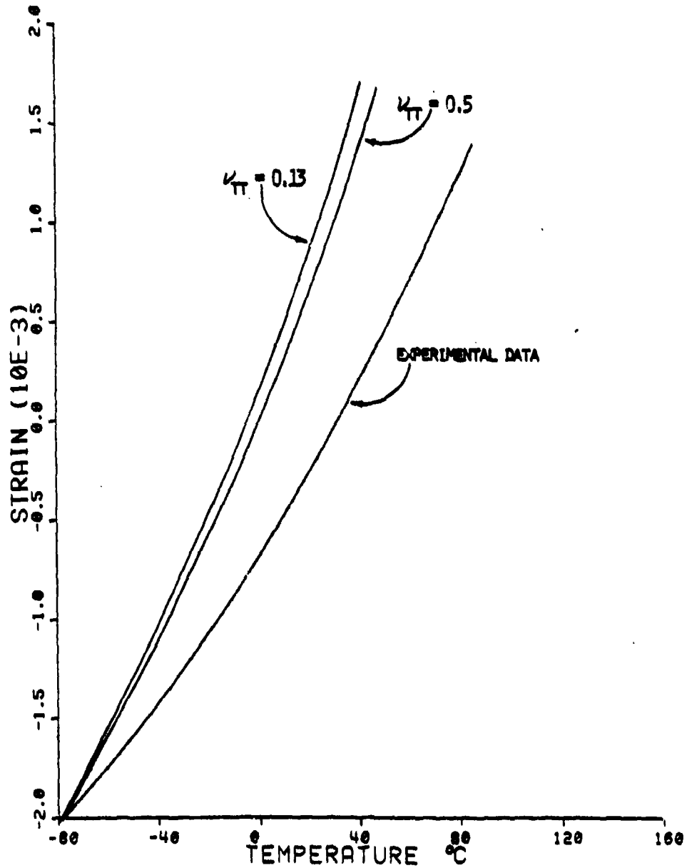
Figure 67. Moisture Conditioned Transverse Thermal Expansion Sensitivity to In-Plane Poisson's Ratio of the Fiber for AS/3901-6 Graphite/Epoxy (Base Value \nu_{TT} = 0.25 )
