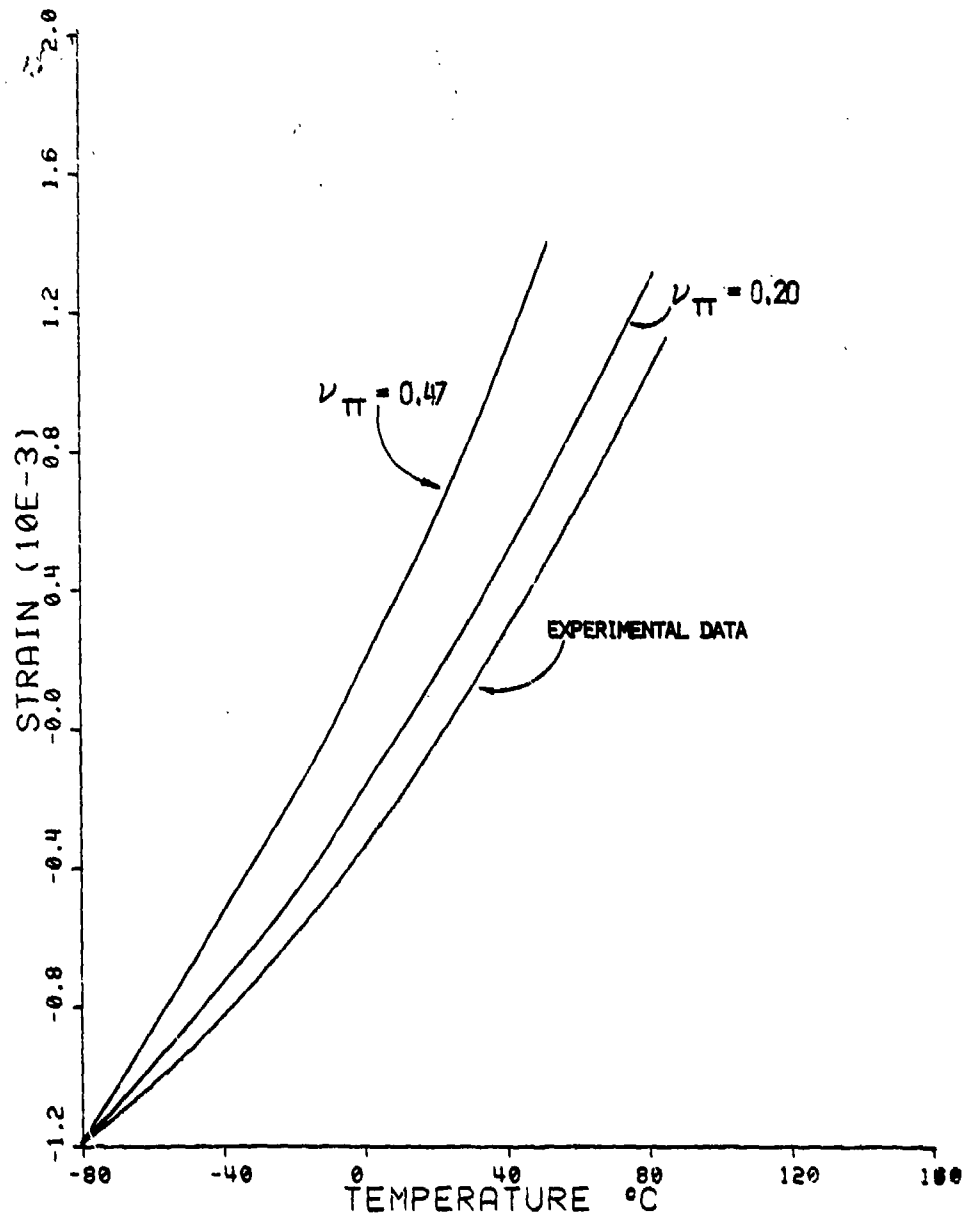
Figure 77. Moisture Conditioned Transverse Thermal Expansion Sensitivity to Poisson's Ratio of the Matrix for S2 Glass/3501-6 Glass/Epoxy (Base Value of Matrix \nu_{\pi} = 0.34 )
