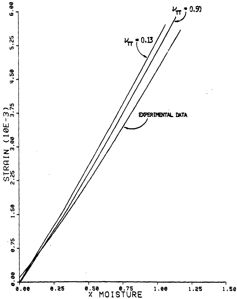
Figure 45. Moisture Expansion Sensitivity to In-Plane Poisson's Ratio of the Fiber for AS/3501-6 Graphite Epoxy (Base Value of Fiber \nu_{TT} = 0.25 )
