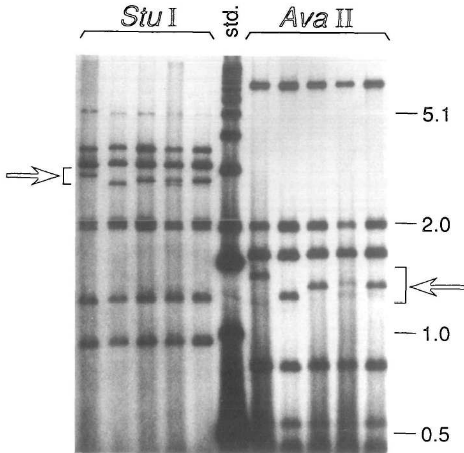
Figure 3. Stu I and Ava II digests of Malaclemys mtDNA. Five individuals are shown, arranged in the same order from left to right in digests for the two enzymes. The regions indicated by arrows exhibit the concordant band shifts resulting from the size polymorphism and heteroplasmy. Numbers refer to selected fragment lengths (kb) of the molecular size standard in the middle lane.
