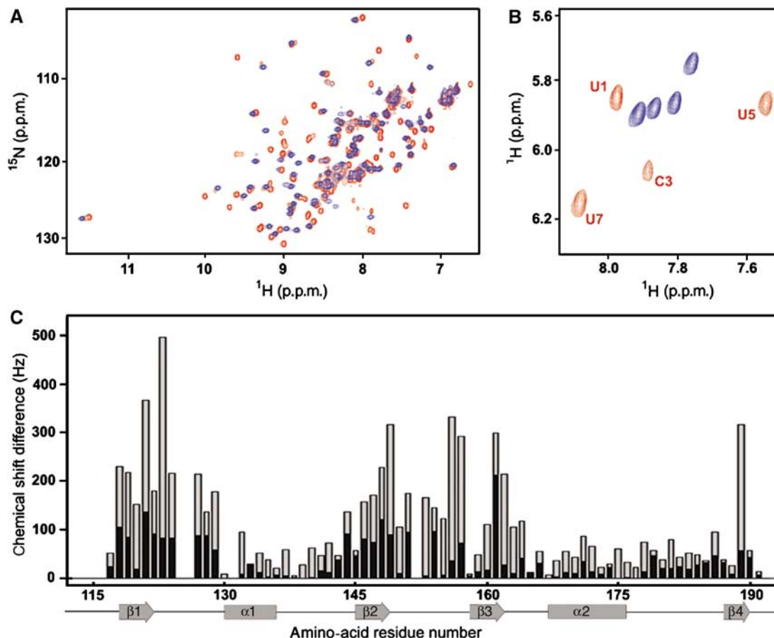
Figure 1 UGCAUGU binds to the RBD of Fox-1 and affects residues in the \beta -sheet and in loops. (A) ^{15}\text{N} -labeled HSQC spectra of \sim 1 mM solutions of the free RBD of Fox-1 (blue) and of the RBD of Fox-1 in the presence of one equivalent of 5'-UGCAUGU-3' (red) at 313 K. (B) Sections of 2D TOCSY spectra showing the H5-H6 correlations of uracil and cytosine of \sim 1 mM solutions of free 5'-UGCAUGU-3' (blue) and of 5'-UGCAUGU-3' in the presence of one equivalent of protein (red). (C) The changes in chemical shift of the backbone amide nitrogen (black) and proton (grey) between free and bound Fox-1 (in Hz, on a 600 MHz spectrometer) are plotted versus the amino-acid residue number. Large chemical shift changes occur in the \beta -strands as well as in loops \beta_1\alpha_1 and \beta_2\beta_3 (assignments for residues 125, 126, 131, 152 and after 191 could not be obtained for the free protein).
