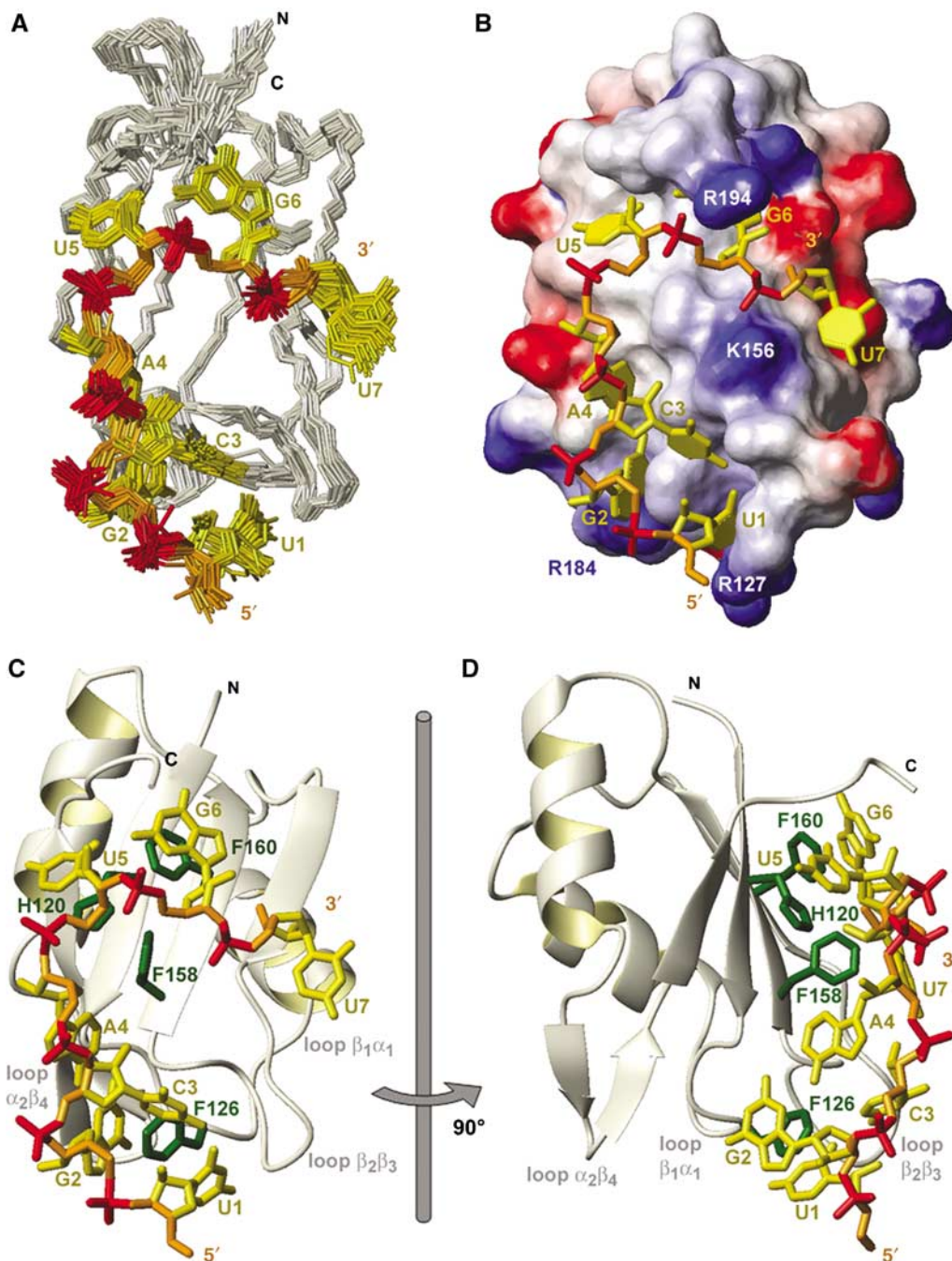
Figure 2 Overview of the solution structure of the RBD of Fox-1 in complex with UGCAUGU. (A) Overlay of the final 30 structures superposed on the heavy atoms of the structured parts of the protein and of the RNA. The protein backbone is gray, the RNA backbone is orange, the phosphate groups are red, and the RNA bases are yellow. Only the ordered region of the protein (residues 116–194) is shown. (B) Surface (heavy atoms of residues 116–194) and stick (heavy atoms of the RNA) representation of the lowest energy structure. The protein surface is painted according to surface potential with red indicating negative charges and blue indicating positive charges. The RNA is colored as in panel (A). (C) The lowest energy structure in ribbon (protein backbone) and stick (RNA) representation. The color scheme is the same as in (A), important protein side chains involved in hydrophobic interactions with the RNA are represented as green sticks. (D) Same as (C) but rotated by 90° around the indicated axis. Figures were generated with MOLMOL (Koradi et al , 1996).
