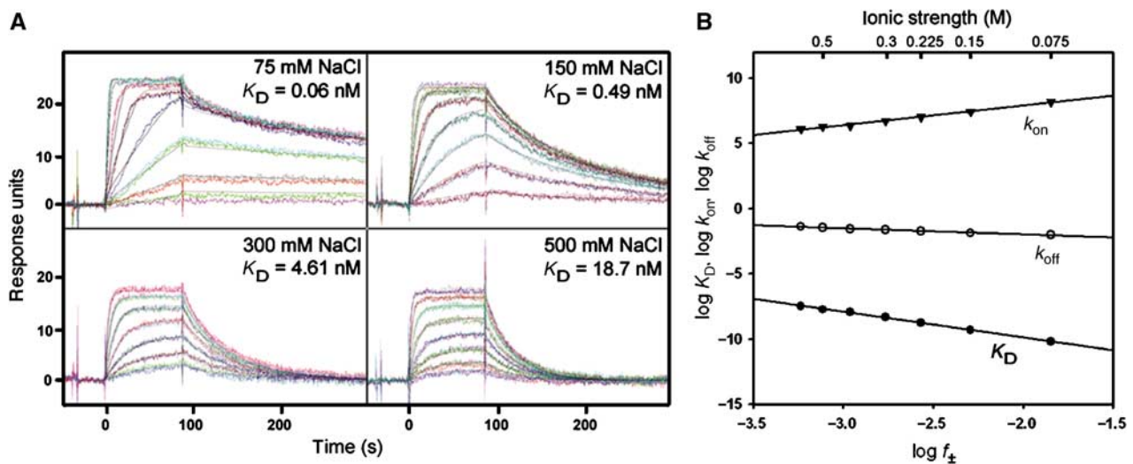
Figure 4 Salt dependence of RNA binding examined by surface plasmon resonance measurements. (A) Representative curves for binding of the RBD of Fox-1 to an immobilized oligonucleotide biotin-5'-CUCUGCAUGU-3' at different salt concentrations. At 75, 150, 300 and 500 mM NaCl, binding curves for 20, 10, 5, 2.5, 1.25, 0.625, 0.312 and 0.156 nM protein, 20, 10, 5, 2.5, 1.25, 0.625 and 0.312 nM protein, 80, 40, 20, 10, 5, 2.5 and 1.25 nM protein, and 320, 160, 80, 40, 20, 10, 5 and 2.5 nM protein are shown, respectively. Curves are fit according to a 1:1 Langmuir interaction model including a correction term for mass transport limitations and are shown as grey lines. (B) Plot of \log K_D (●), \log k_{off} (○) and \log k_{on} (▲) versus \log f_{\pm} . f_{\pm} is the electrostatic contribution to the mean rational activity coefficient, which is linked to the ionic strength, see Materials and methods section and Supplementary Table SII. Each data point represents the average of at least three independent measurements.
