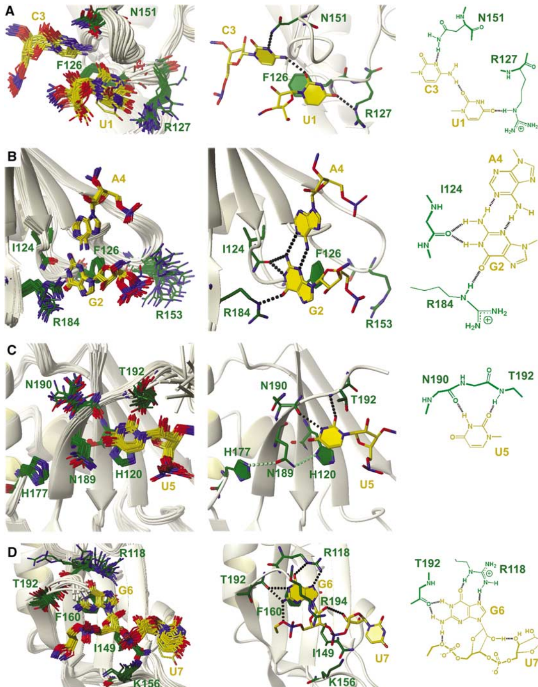
Figure 3 Molecular recognition of UGCAUGU by the RBD of Fox-1. Close-up views of the RNA binding interface of the overlay of the final 30 structures superposed on the heavy atoms of the structured parts of the protein and of the RNA (left), single structures showing the intermolecular and intra-RNA interactions that are most commonly observed in the 30 structures (middle; see Supplementary Table S1) and schematic representations of the hydrogen bonding interactions that are most commonly observed in the 30 structures (right). The ribbon representation of the protein backbone is shown in grey, side chains of the protein are in green and the RNA is in yellow. Recognition of U 1 and C 3 (A), of G 2 and A 4 (B), of U 5 (C), and of G 6 and U 7 (D). Figures were generated with MOLMOL (Koradi et al , 1996).
