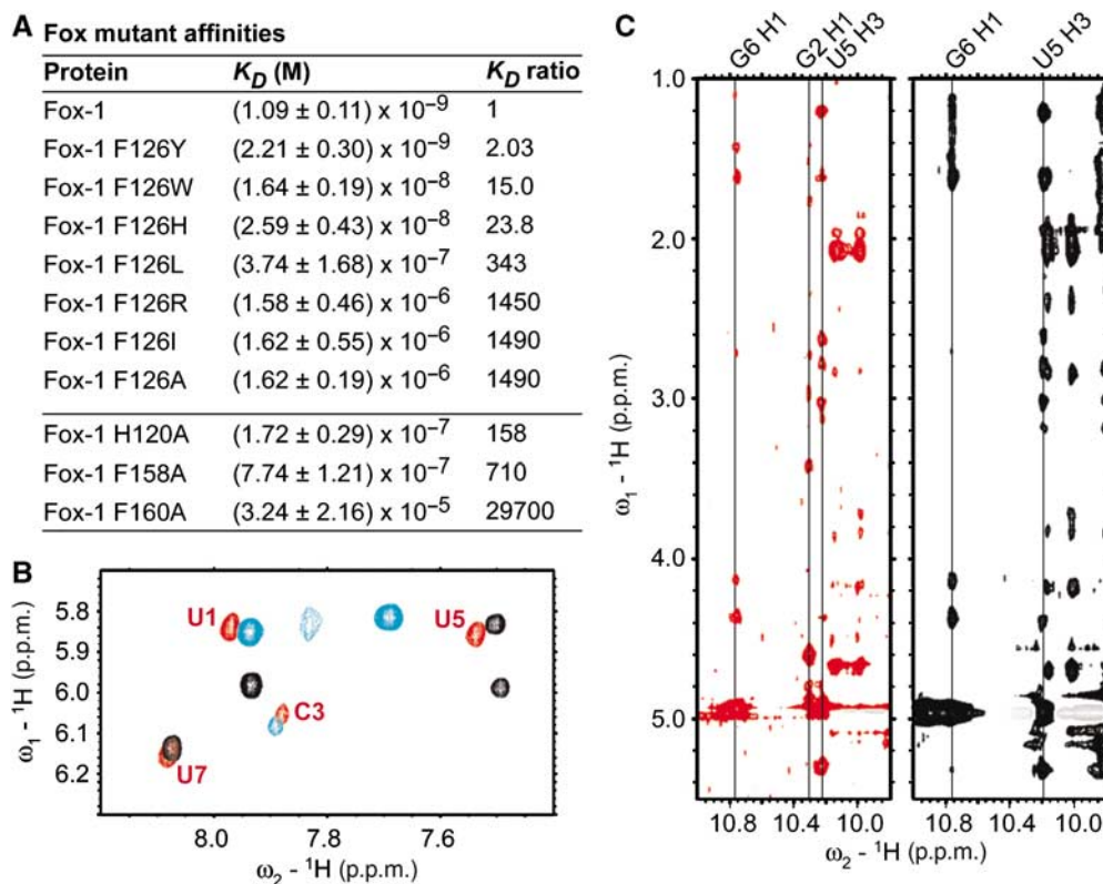
Figure 5 F126 plays a crucial role in RNA binding. (A) Affinities of single amino-acid mutants of Fox-1. Values for K_D s are derived from steady state binding levels at different protein concentrations using surface plasmon resonance. Each measurement was repeated three times at 150 mM NaCl and pH 7.4. (B) Overlay of sections of 2D TOCSY spectra showing the H5-H6 correlations of uracil and cytosine of \sim 1 \text{ mM} solutions of 5'-UGCAUGU-3' in the presence of one equivalent of Fox-1 (red), Fox-1 F126A (black), and Fox-1 F160A (cyan). (C) Sections of 2D NOESY spectra of a 1:1 complex of Fox-1 (red) or Fox-1 F126A (black) with UGCAUGU showing NOE crosspeaks to the imino protons of G6, G2 and U5.
