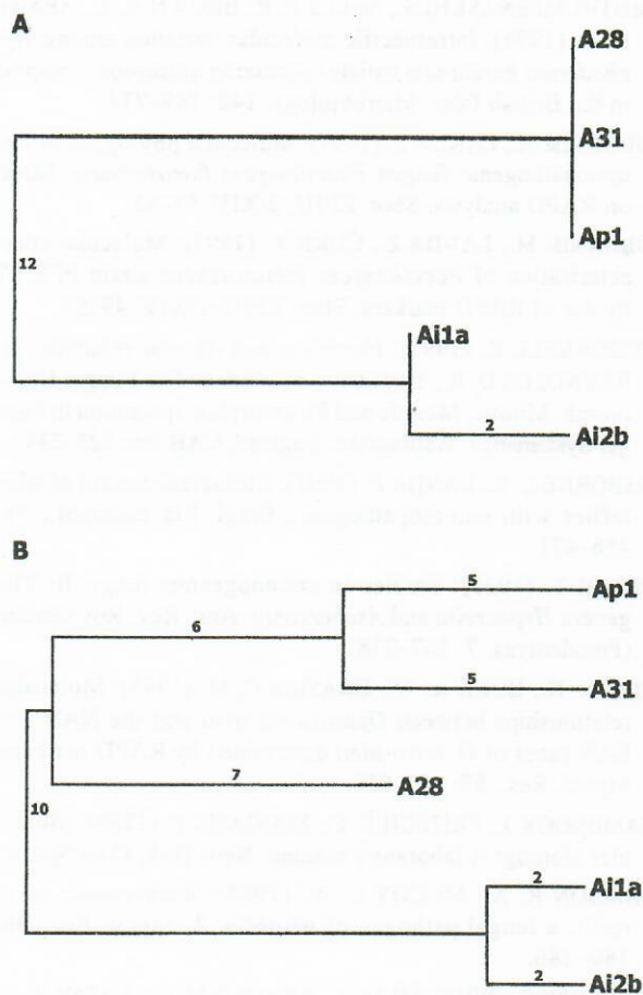
Fig. 3. Phylogenetic trees of five Aschersonia isolates inferred from 26S rDNA sequences (A) and RAPD data (B). Type of trees – phylogram. Numbers on the trees branches indicates number of characteristics supporting each branching (PAUP 3.1.1. Heuristic options, SWOFFORD 1993)
