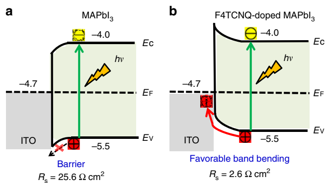
Fig. 4 Interfacial hole transfer dynamics. Schematic illustrations of hole transfer at the a ITO/MAPbI 3 or b ITO/F4TCNQ-doped MAPbI 3 interface
