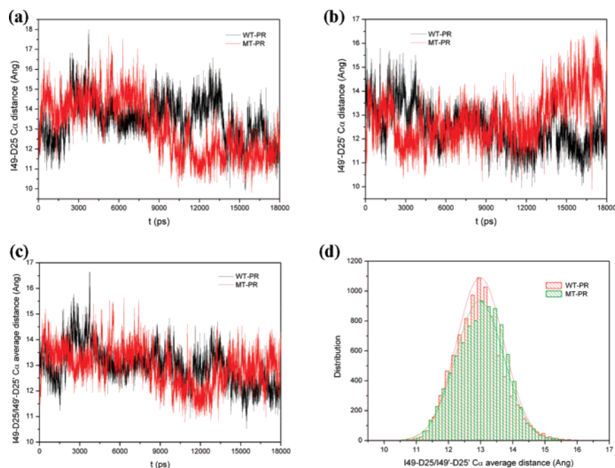
Figure 10. Variability of (a) the I49-D25 C _{\alpha} distances, (b) the I49'-D25' distances, and (c) the I49-D25/I49'-D25' average distance of the unbound wild-type protease (WT-PR) and the unbound mutated protease (MT-PR). (d) Histogram distributions of the average distance in Figure 10c.
