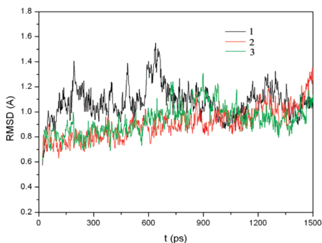
Figure 2. Root-mean-square displacement (rmsd) of the backbone C _{\alpha} atoms of the wild-type HIV-1 protease/ 1 complex, the wild-type HIV-1 protease/ 2 complex, and the wild-type HIV-1 protease/ 3 complex with respect to the first snapshot as a function of time.
