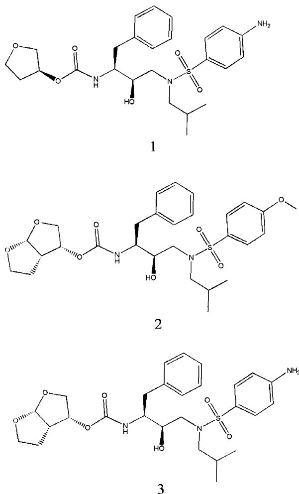
Figure 1. Chemical structures of 1 , 2 , and 3 .
