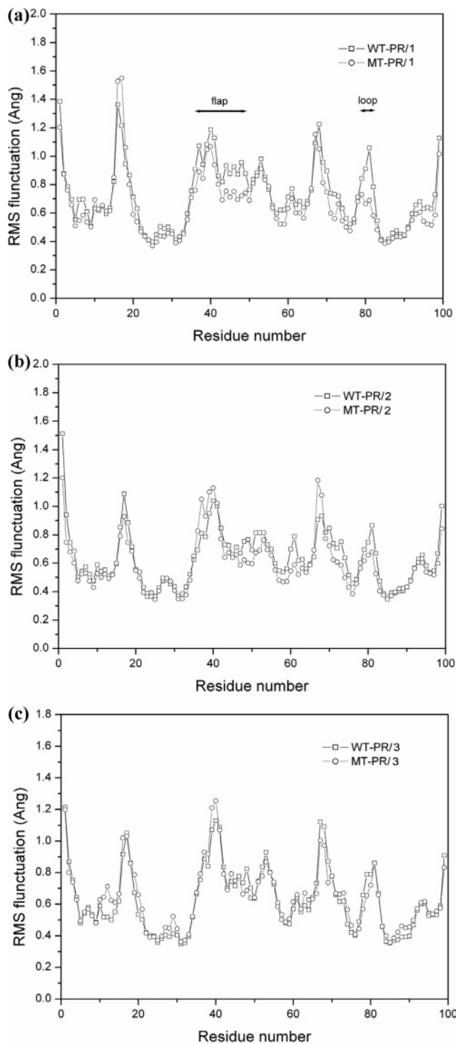
Figure 12. Root-mean-square fluctuation of backbone atoms versus residue number for both monomers of (a) the wild-type HIV-1 protease/ 1 complex and the mutated HIV-1 protease/ 1 complex, (b) the wild-type HIV-1 protease/ 2 complex and the mutated HIV-1 protease/ 2 complex, and (c) the wild-type HIV-1 protease/ 3 complex and the mutated HIV-1 protease/ 3 complex.
