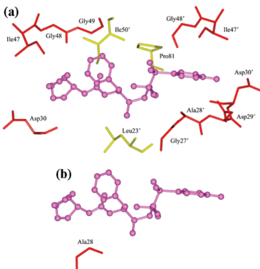
Figure 6. (a) Geometries of ten residues that contribute most to the difference between the van der Waals interaction of 1 and that of 3 . The residues with stronger van der Waals interaction with 3 are colored in red, and those with weaker van der Waals interaction with 3 in yellow. (b) Geometries of four residues that contribute most to the difference between the electrostatic interaction and the polar contribution of solvation of 1 and that of 3 . The residues with the stronger electrostatic interaction and polar contribution of solvation with 3 are colored in red, and those with the weaker in blue. The structure of 3 is shown in purple ball-and-stick model.
