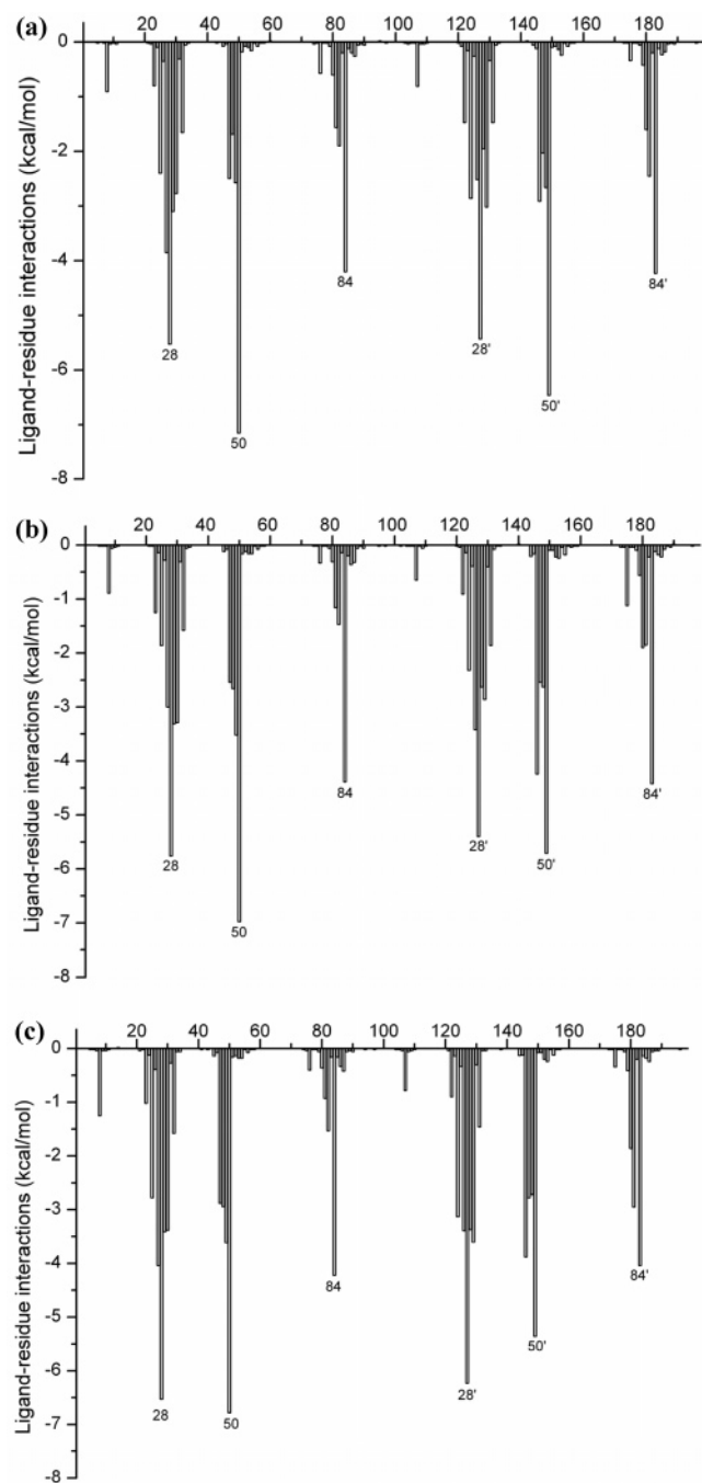
Figure 4. Ligand-residue interaction spectrum of (a) the HIV-1 protease/1 complex, (b) the HIV-1 protease/2 complex, and (c) the HIV-1 protease/3 complex according to the MM/GBSA method. The x -axis denotes the residue number of PR and the y -axis denotes the interaction energy between the inhibitor and specific residues.
