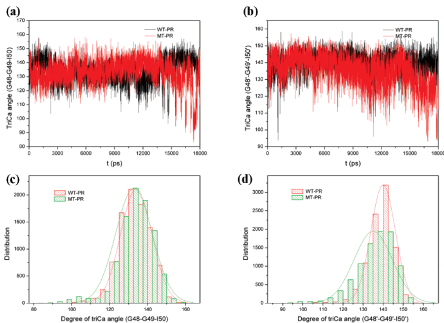
Figure 9. Variability of (a) the G48-G49-I50 triC _{\alpha} angle and (b) the G48'-G49'-I50' triC _{\alpha} angle of the unbound wild-type protease (WT-PR) and the unbound mutated protease (MT-PR). Histogram distributions of (c) the G48-G49-I50 triC _{\alpha} angle and (d) the G48'-G49'-I50' triC _{\alpha} angle.
