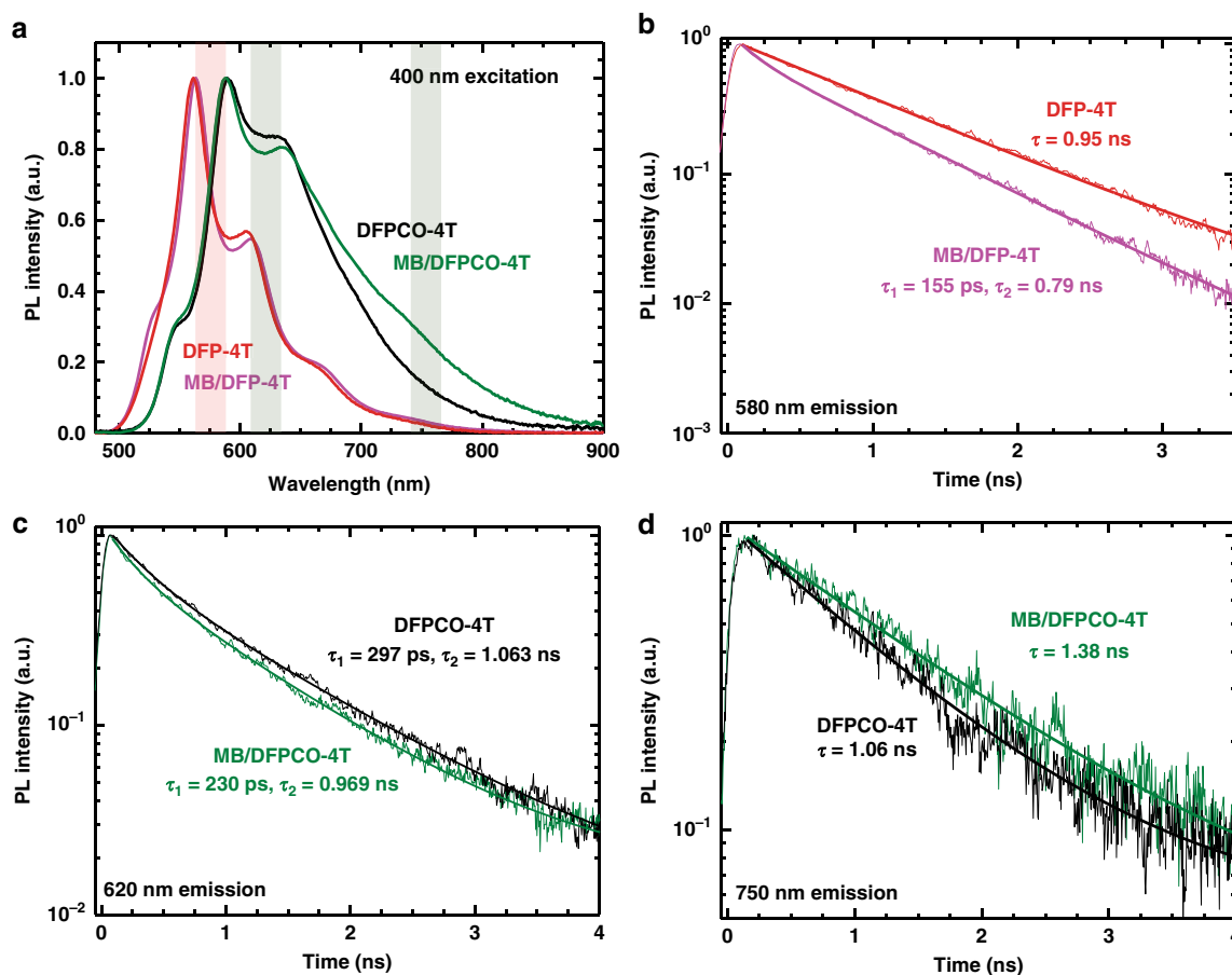
Fig. 4 Photoluminescence spectroscopy measurements. a Steady-state and ( b–d ) transient photoluminescence of films upon 400 nm excitation (The shaded areas in a indicate the spectral regions wherein PL dynamics were investigated in b–d ). The steady state spectra of the DFP-4T system are virtually identical in both cases ( a ), but a quicker decay of the main emission in the transients of MB/ DFP-4T points to a charge transfer towards MB ( b ). The DFPCO-4T system shows a marked increase in the PL around 750 nm upon MB deposition. The main emission occurs slightly faster c for MB/ DFPCO-4T , but significantly slower in the tail region d .
