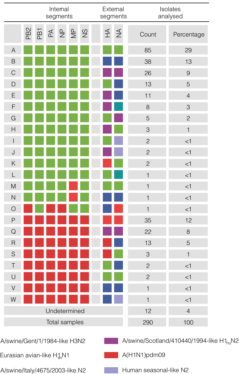
FIG 1 swIAV genotypes isolated from European swine between 2009 and 2013. The 23 distinct genetic constellations are labeled A to W, with the lineage of origin for each segment indicated by a colored block.
