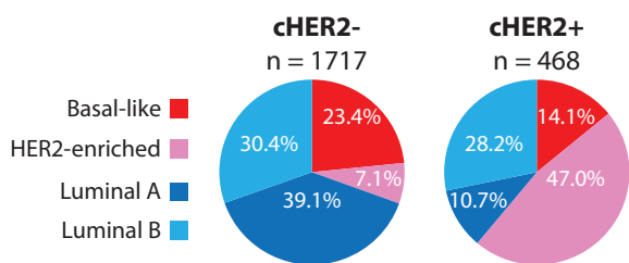
Figure 1. Distribution of the intrinsic molecular subtypes of breast cancer in clinical HER2 status (cHER2)-negative and cHER2+ disease in the combined the cancer genome atlas and molecular taxonomy of breast cancer international consortium dataset. cHER2 = clinical HER2 status.
