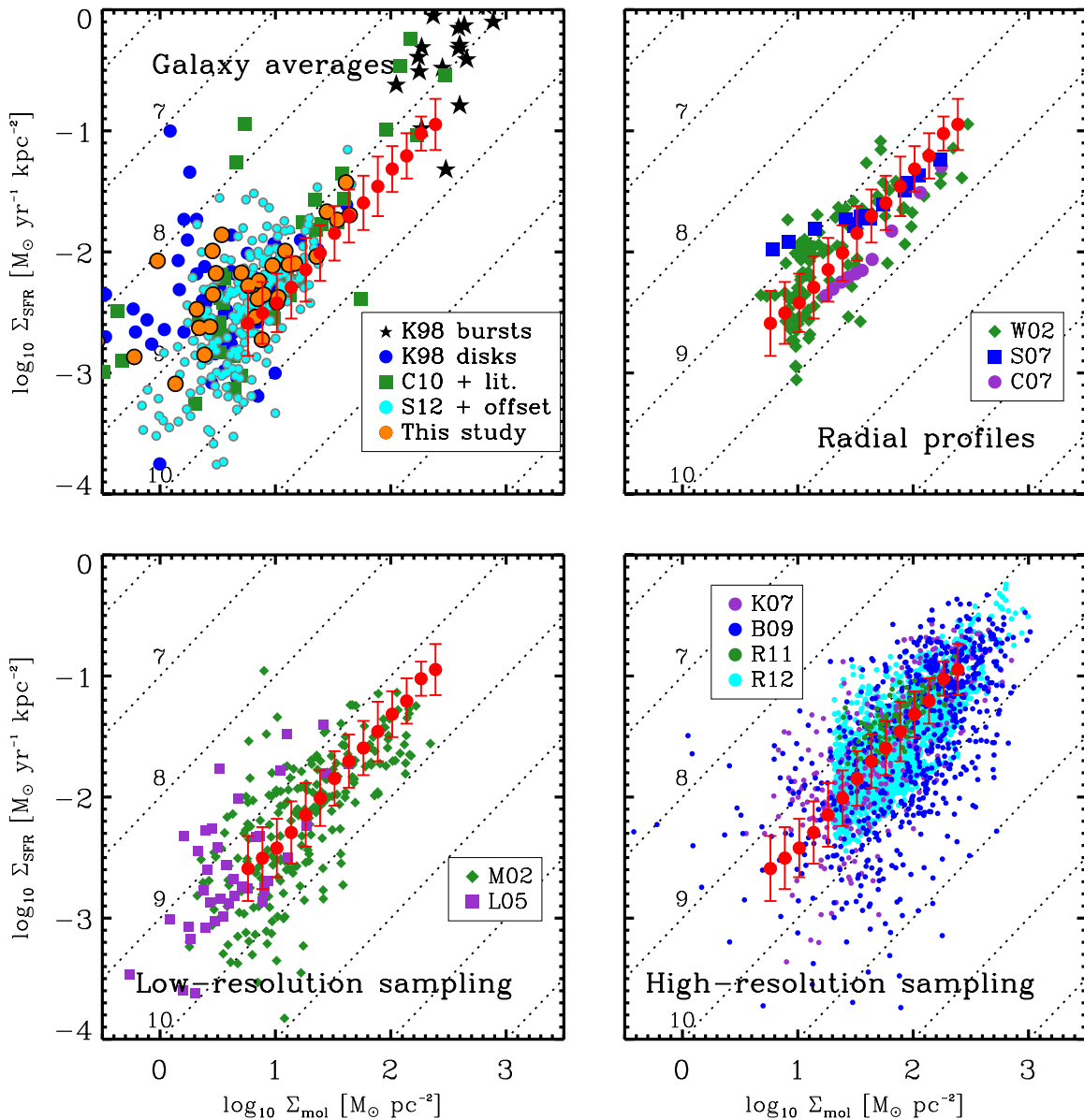
Figure 6. \Sigma_{\text{SFR}} vs. \Sigma_{\text{mol}} for our results and literature measurements. The type of literature measurement varies with panel: the top left shows galaxy averages, the top right shows radial profiles, the lower left shows sparse, coarse ( \sim 1' ) sampling of galaxy disks, and the lower right shows fine sampling ( \lesssim 15'' ). In all four panels, red points show a running median and standard deviation (error bars) for our kpc-scale measurements (Figure 1) using \text{H}\alpha + 24\ \mu\text{m} and CO (2–1). Orange circles in the top left panel show integrated measurements for our data. Literature measurements are described in Section 2. References. K98: Kennicutt (1998a); C10 + lit.: Calzetti et al. (2010) combined with literature CO; S12: Saintonge et al. (2012) with offset to bring SFR estimates into agreement (Section 2.2); W02: Wong & Blitz (2002); S07: Schuster et al. (2007); C07: Crosthwaite & Turner (2007); M02: Murgia et al. (2002); L05: Leroy et al. (2005); K07: Kennicutt et al. (2007); B09: Blanc et al. (2009); R11: Rahman et al. (2011); R12: Rahman et al. (2012).
