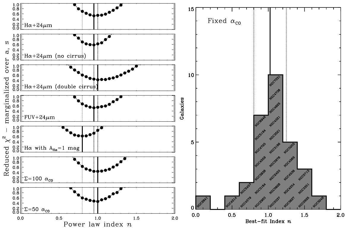
Figure 5. Results of power-law fitting for (left) our combined data set and (right) individual galaxies. Left: goodness of fit as a function of power-law index, n , for fits to our entire ensemble of data where \Sigma_{\text{mol}} > 5 M_{\odot} \text{pc}^{-2} . The fitting uses a modified version of the Monte Carlo technique outlined by Blanc et al. (2009). From top to bottom, we show results for fixed \alpha_{\text{CO}} using our best \text{H}\alpha+24\mu\text{m} and \text{FUV}+24\mu\text{m} estimates; \text{H}\alpha+24\mu\text{m} with no cirrus removed or double the best-estimate cirrus removed; and \text{H}\alpha with an assumed fixed 1 magnitude of extinction. We also show results for our “ \Sigma = 100 ” and “ \Sigma = 50 ” conversion factors. Vertical lines indicate where n reaches its minimum value, bold for the value in that panel, dotted for other panels. Each case shows a broad minimum in \chi^2 with a best-fit value near n \approx 1 \pm 0.2 . Right: best-fit power-law index, n , for individual galaxies using \text{H}\alpha+24\mu\text{m} and a fixed \text{CO} -to- \text{H}_2 conversion factor. The distribution of best-fit n for individual galaxies peaks near n \approx 1 with most galaxies in the range n \approx 0.8 – 1.2 but outliers up to n \gtrsim 1.5 .
