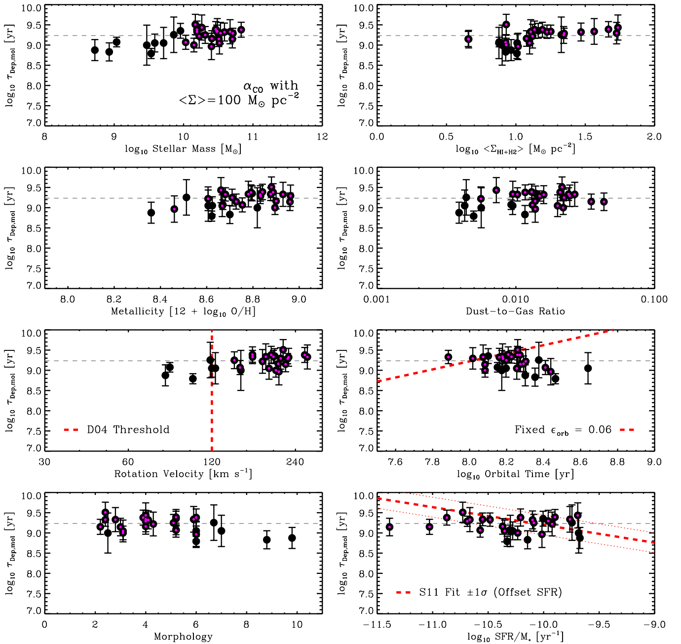
Figure 8. Same as Figure 7 but after application of our variable “ \Sigma = 100 ” CO-to-H 2 conversion factor. Most of the galaxy-scale variations in \tau_{\text{dep}}^{\text{mol}} visible in Figure 7 can largely be explained by this dust-to-gas ratio-dependent conversion factor, though significant galaxy-to-galaxy scatter remains. A dashed horizontal line in each panel shows the median \tau_{\text{dep}}^{\text{mol}} across our sample, and we reproduce several comparison lines from Figure 7.
