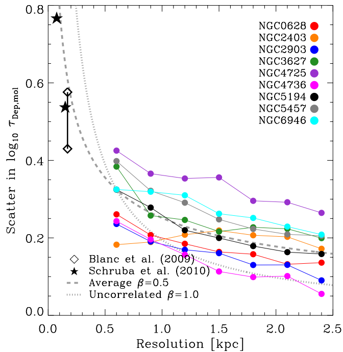
Figure 12. Evidence for spatial correlation among \tau_{\text{dep}}^{\text{mol}} within galaxies. We plot rms scatter in \log_{10} \tau_{\text{dep}}^{\text{mol}} (y-axis) as a function of spatial resolution (x-axis) for a subset of nearby, large galaxies. The scatter in \tau_{\text{dep}}^{\text{mol}} changes more slowly as a function of resolution than one would expect averaging uncorrelated data. Extrapolating the trend that we observe to much higher resolution yields reasonable consistency with (scarce) high-resolution literature data (Blanc et al. 2009; Schrubba et al. 2010). We illustrate the median trend, \beta = 0.5 , while \beta = 1 would be expected for a disk filled with uncorrelated star-forming regions. This low \beta reflects systematic variations in \tau_{\text{dep}}^{\text{mol}} on intermediate scales, either due to synchronization of star formation on intermediate scales (e.g., see Feldmann et al. 2011) or systematic but still undiagnosed environment dependencies of the efficiency of star formation.
