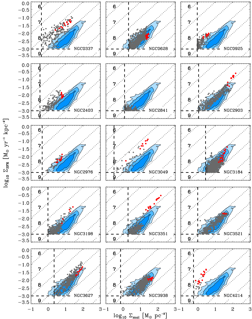
Figure 18. \Sigma_{\text{SFR}} , estimated from \text{H}\alpha+24\mu\text{m} , as a function of \Sigma_{\text{mol}} , estimated from HERACLES CO (2–1) data and a fixed \alpha_{\text{CO}} , for individual galaxies. Data from the designated galaxy appear in gray, with data from the inner 0.1r_{25} marked in red. In the background, we plot data density contours from the ensemble of all measurements (Figure 1). Annotation and symbols are otherwise as Figure 1.
