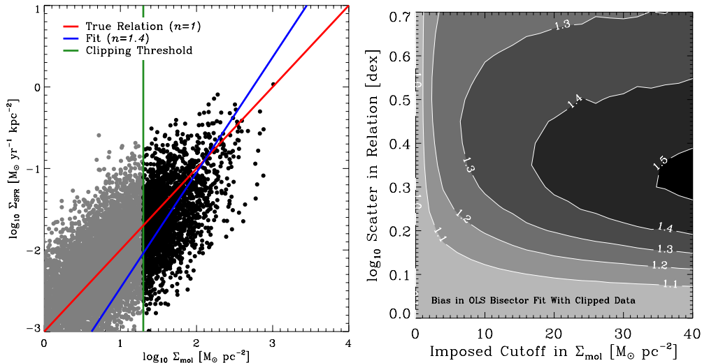
Figure 17. Left: example of the biases introduced by clipping data on one axis (e.g., due to limited S/N) before carrying out a bivariate fit. Points show a simulated data set in which \Sigma_{\text{SFR}} \propto \Sigma_{\text{mol}} by construction (red line) with 0.3 dex scatter introduced to each axis. We clip data below \Sigma_{\text{mol}} = 20 M_{\odot} \text{pc}^{-2} so that gray points are discarded and black points are fit. We then fit the black points using the OLS bisector method and plot the result in blue. The result is a bias toward higher slope. Right: derived power-law index from using the OLS bisector to fit noisy, low dynamic range data with clipping applied to one axis. The underlying model has an intrinsic n = 1.0 slope with \Sigma_{\text{mol}} drawn from our data and log-normal scatter of the indicated magnitude applied to each axis. The gray scale and contours report the best-fit power-law index after the data are clipped at the x -axis value in one axis and fit using the OLS bisector technique. Biases of several tenths up to as much as four tenths are possible within the range of values adopted by recent studies.
