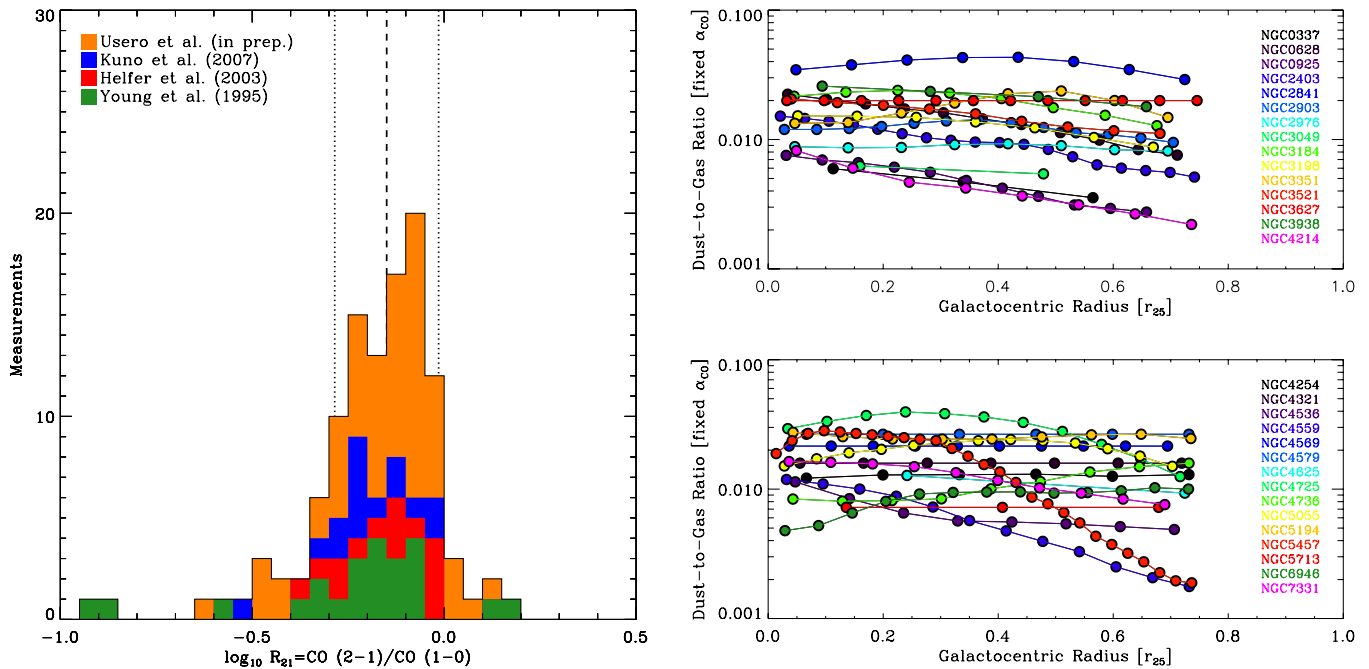
Figure 15. Line ratios and dust-to-gas ratios in HERACLES. Left: CO (2–1)/CO (1–0) line ratio comparing HERACLES integrated measurements to literature CO (1–0) surveys: Kuno et al. (2007), Helfer et al. (2003), Young et al. (1995), and measurements for individual pointings obtained for follow-up spectroscopy by A. Usero et al. (in preparation). The ensemble of measurements has median 0.67 with scatter 0.16 dex. Right: dust-to-gas ratio profiles derived comparing IR SED modeling, HERACLES, and H I data. We plot the radial profile of the dust-to-gas ratio derived using a fixed conversion factor.
