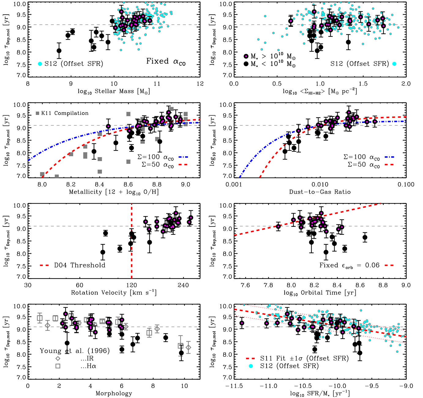
Figure 7. Integrated \tau_{\text{dep}}^{\text{mol}} ( \Sigma_{\text{mol}}/\Sigma_{\text{SFR}} ) within 0.75r_{25} and standard deviation (error bars) in \tau_{\text{dep}}^{\text{mol}} over individual lines of sight plotted against integrated galaxy properties: stellar mass, average gas mass surface density, metallicity, dust-to-gas mass ratio, rotation velocity at r_{25} , orbital period at 0.4r_{25} , morphology, and specific SFR ( \Sigma_{\text{SFR}}/\langle\Sigma_{*}\rangle ). Literature data appear in gray (Y96, K11, and S12 refer to Young et al. 1996; Krumholz et al. 2011; Saintonge et al. 2012), and fits or predictions appear as curves: Wolfire et al. (2010) conversion factors for \Sigma = 50 and 100 M_{\odot} \text{pc}^{-2} , the rotation-velocity threshold associated with the suppression of dust lanes by Dalcanton et al. (2004, D04), a fixed efficiency per orbital period, and the \tau_{\text{dep}}^{\text{mol}} vs. SFR fit by Saintonge et al. (2011, S11). Low-mass, metal-poor, late-type galaxies show significantly lower \tau_{\text{dep}}^{\text{mol}} (high SFR-to-CO ratios) than their massive, early-type counterparts, but these trends persist with smaller dynamic range even among massive galaxies (we mark galaxies with M_{*} > 10^{10} M_{\odot} using magenta dots in all panels).
