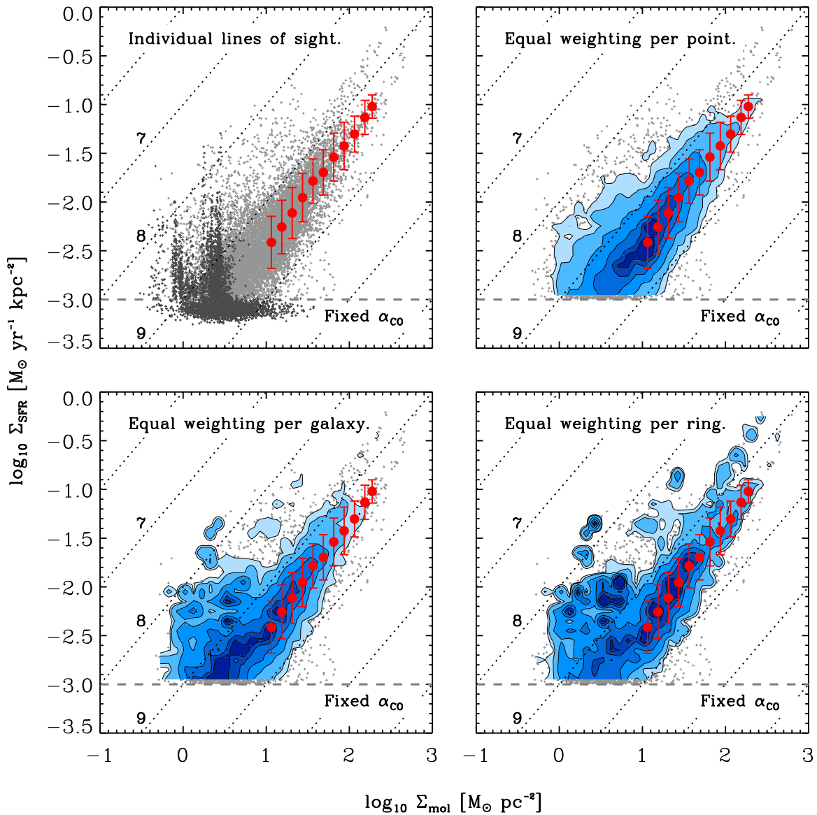
Figure 1. Star formation rate surface density, \Sigma_{\text{SFR}} , estimated from \text{H}\alpha+24\mu\text{m} emission, as a function of molecular gas surface density, \Sigma_{\text{mol}} , derived from CO (2–1) emission for 30 nearby disk galaxies. The top left panel shows individual points (dark gray points show upper limits) with the running median and standard deviation indicated by red points and error bars. The red points with error bars from the first panel appear in all four panels to allow easy comparison. Dotted lines indicated fixed \text{H}_2 depletion times; the number indicates \log_{10} \tau_{\text{dep}} in yr. The top right panel shows the density of the data in the top left panel. In the bottom panels we vary the weighting used to derive data density. The bottom left panel gives equal weight to each galaxy. The bottom right panel gives equal weight to each galaxy and each radial bin.
