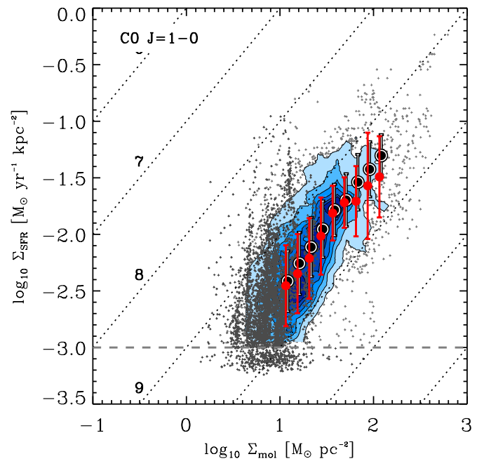
Figure 3. Star formation rate surface density, \Sigma_{\text{SFR}} , as a function of molecular gas surface density, \Sigma_{\text{mol}} , here estimated from literature CO (1–0) data (Section 2). Gray points show individual measurements, contours indicate data density, and red points show the running median and standard deviation using each tracer. For comparison, large black-and-white circles show the same bins from Figure 1.
