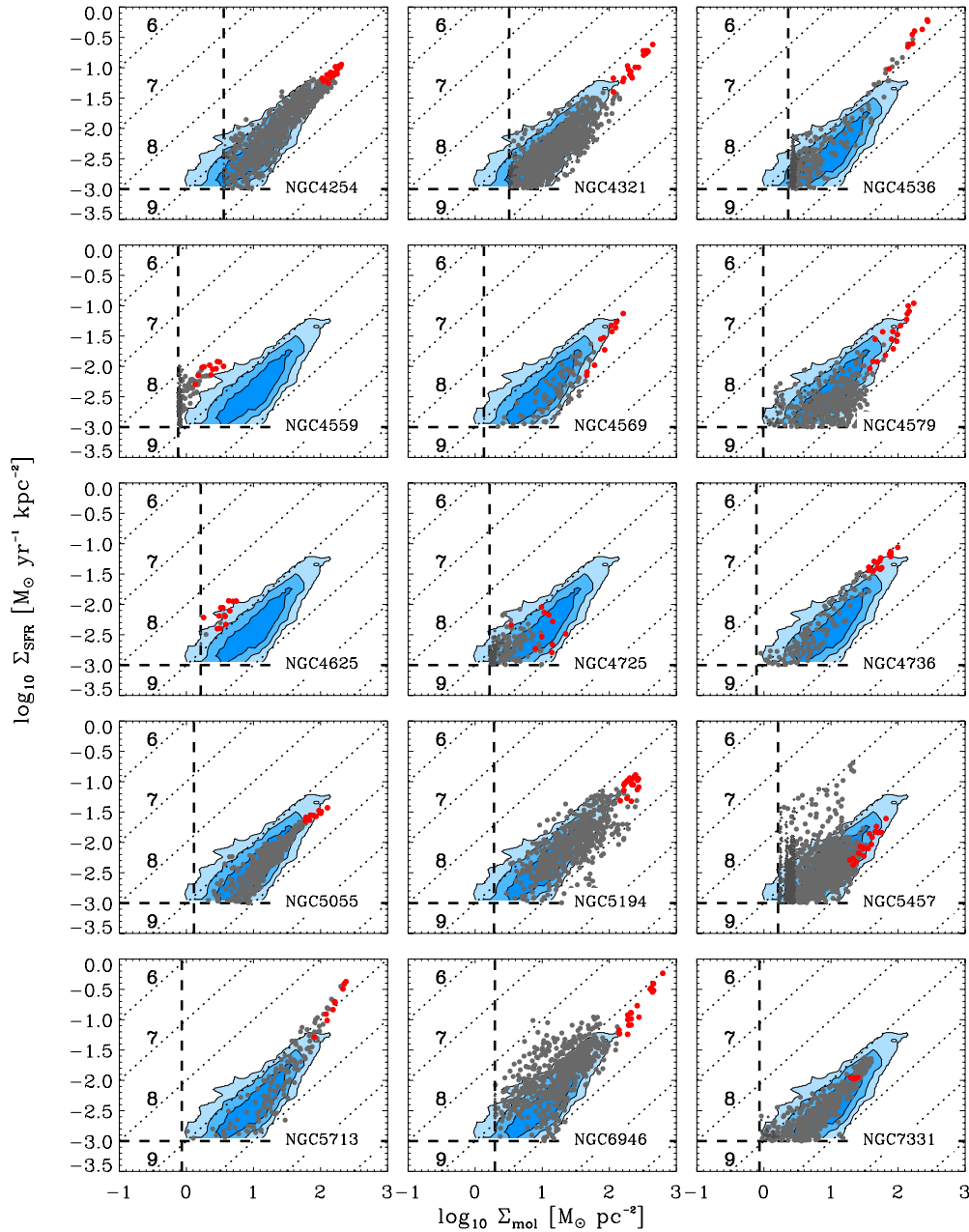
Figure 19. As Figure 18 for the remaining galaxies in our sample.
