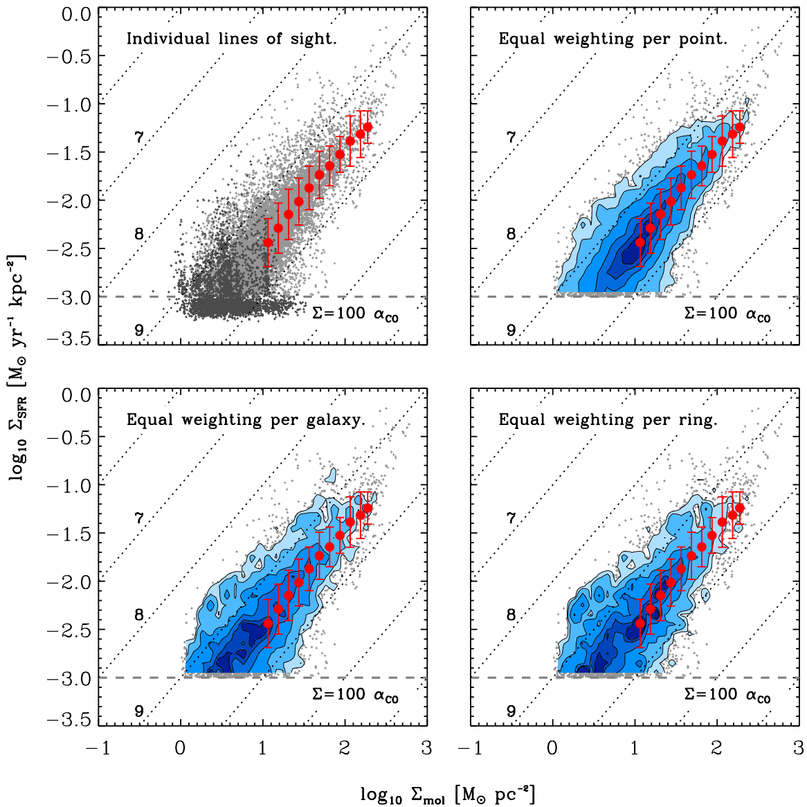
Figure 4. Star formation rate surface density, \Sigma_{\text{SFR}} , as a function of molecular gas surface density, \Sigma_{\text{mol}} , here estimated from CO (2–1) data combined with our “ \Sigma = 100 ” conversion factor \alpha_{\text{CO}} , which reflects variations in the dust-to-gas ratio and the central depressions in \alpha_{\text{CO}} found by Sandstrom et al. (2012). Panels and annotations are as in Figure 1.
