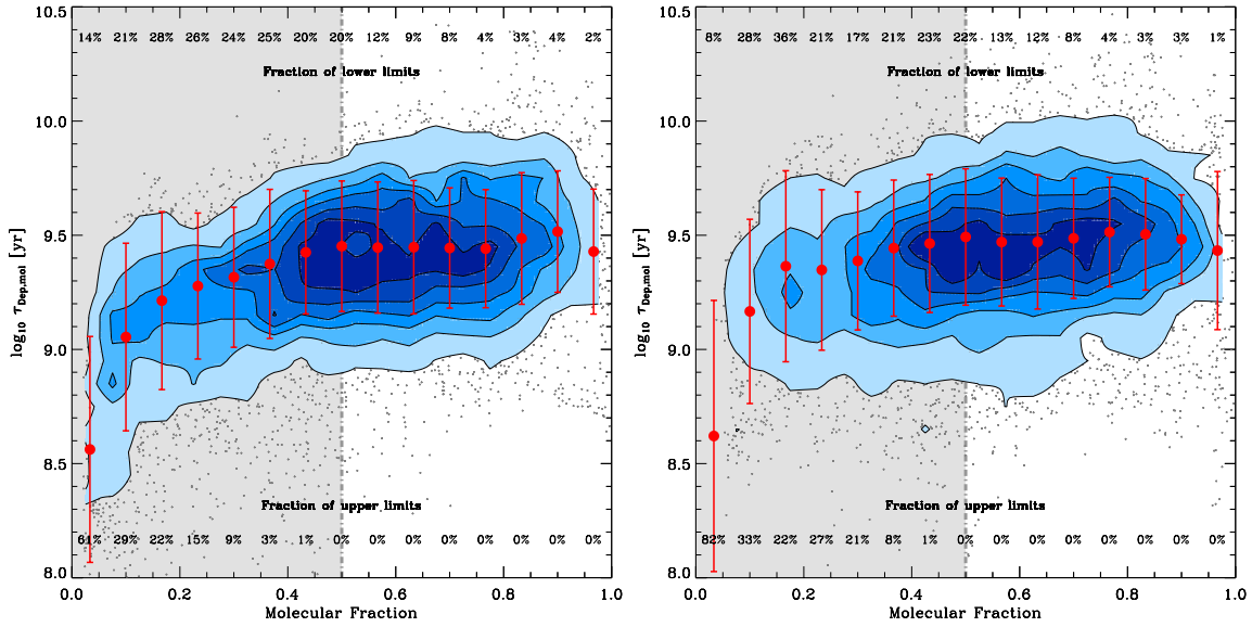
Figure 11. As Figure 9 but showing the molecular gas depletion time, \tau_{\text{dep}}^{\text{mol}} , as a function of the molecular fraction for (left) a fixed \alpha_{\text{CO}} and (right) our “ \Sigma = 100 ” \alpha_{\text{CO}} .
