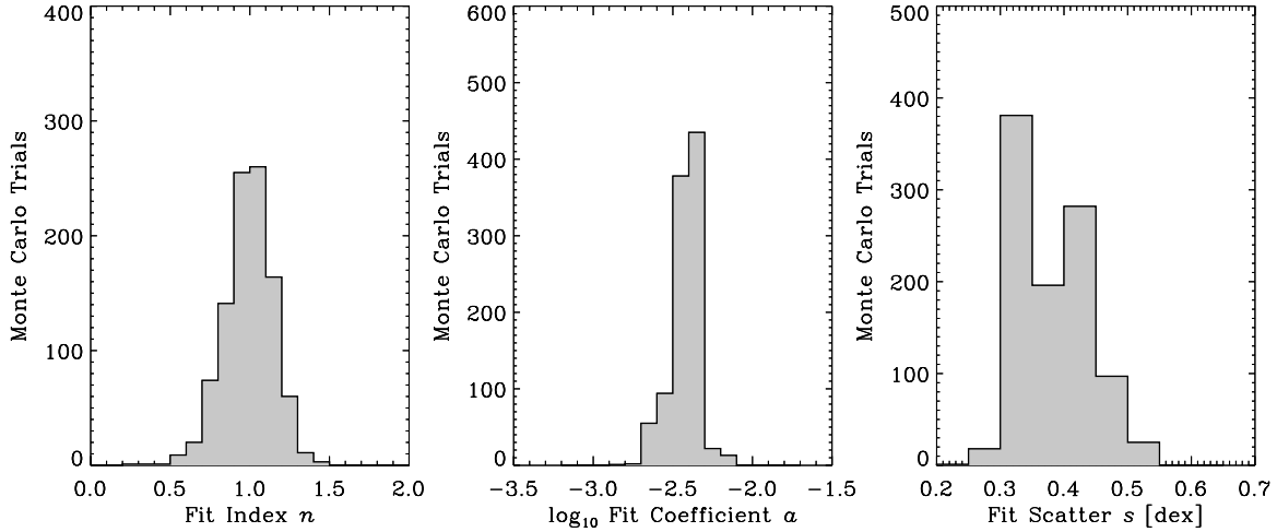
Figure 16. Distribution of best-fit parameters for 1000 Monte Carlo iterations designed to test the impact of observation uncertainties, sample definition, and fitting technique on the best-fit power-law. We plot the distributions of slope n , coefficient a , and intrinsic scatter s across all iterations for our best \Sigma_{\text{SFR}} estimate ( \text{H}\alpha+24\ \mu\text{m} ) and a fixed \alpha_{\text{CO}} .
