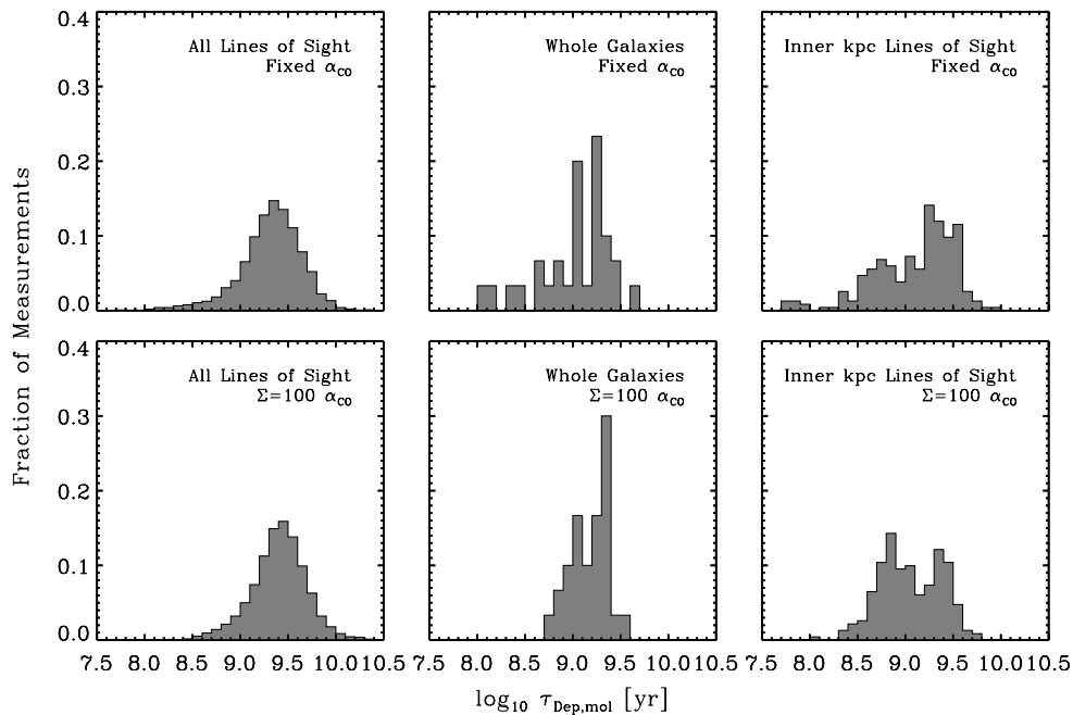
Figure 14. Distribution of molecular gas depletion time, \tau_{\text{dep}}^{\text{mol}} , in HERACLES. We show histograms for all lines of sight at kpc resolution (left), whole galaxies (middle), and lines of sight in the central kpc of our targets (right). The top row shows results for fixed \alpha_{\text{CO}} while the bottom row applies our “ \Sigma = 100 ” conversion factor, which accounts for variable dust shielding and central \alpha_{\text{CO}} depressions. The distribution of \tau_{\text{dep}}^{\text{mol}} treating lines of sight equally appears log-normal, with a depletion time 1–3 Gyr, depending on the adopted conversion factor, and \lesssim 0.3 dex scatter, though low- \tau_{\text{dep}}^{\text{mol}} excursions from the log-normal distribution are already visible in this panel. The distribution of \tau_{\text{dep}}^{\text{mol}} for whole galaxies shows more scatter for a fixed \alpha_{\text{CO}} , reflecting systematic trends in which low-mass, low-metallicity, high-sSFR galaxies show faint CO relative to SFR tracers. After accounting for varying \alpha_{\text{CO}} , there is less scatter among galaxies but some spread remains. Meanwhile the inner kpc of our targets shows a much broader, much less normal distribution, with both low and high \tau_{\text{dep}}^{\text{mol}} common. Correcting for the central \alpha_{\text{CO}} depressions observed by Sandstrom et al. (2012) and expected from observed line ratio variations exacerbates this effect, but it is clearly present even adopting fixed \alpha_{\text{CO}} . Thus, \tau_{\text{dep}}^{\text{mol}} appears constant to first order, but clear systematic second-order variations do emerge as a function of local and galaxy scale conditions in a broad sample.
