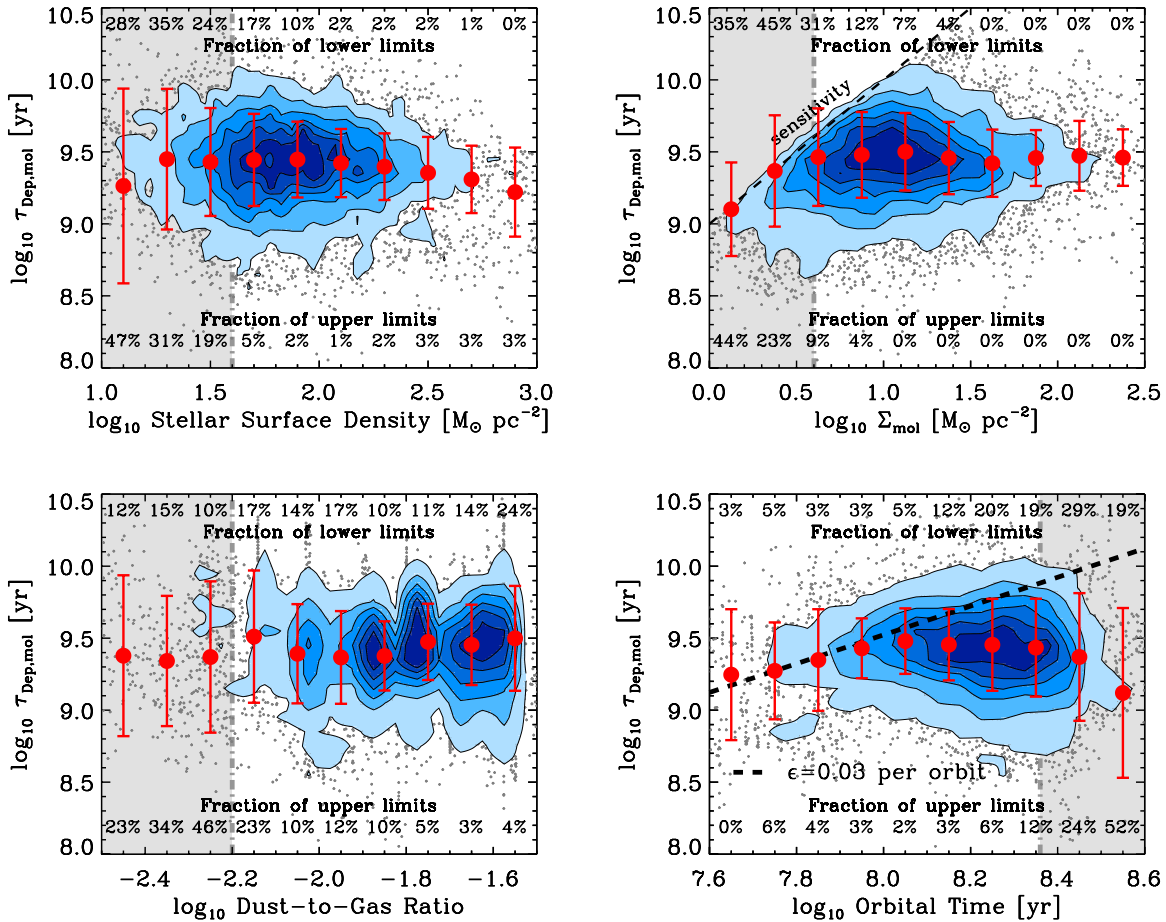
Figure 10. As Figure 9 but after application of our “ \Sigma = 100 ” conversion factor following Wolfire et al. (2010; Equation (4)). The conversion factor correction removes the strongest visible trend in the data.
