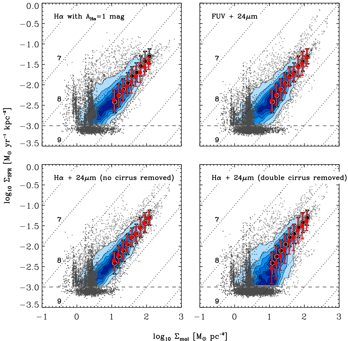
Figure 2. Star formation rate surface density, \Sigma_{\text{SFR}} , estimated using different tracers as a function of molecular gas surface density, \Sigma_{\text{mol}} . Light gray points show individual measurements, dark gray points indicate upper limits, contours show data density, and red points show the running median and standard deviation using each tracer. For comparison, black-and-white points show the bins from the top right panel of Figure 1. We show \Sigma_{\text{SFR}} estimated from H \alpha assuming 1 magnitude of extinction (top left), a combination of FUV and 24 \mu\text{m} emission (top right; L12), H \alpha combined with 24 \mu\text{m} emission with no IR cirrus correction applied to the 24 \mu\text{m} (bottom left), and H \alpha combined with 24 \mu\text{m} with double our IR cirrus correction applied to the 24 \mu\text{m} (bottom right).
