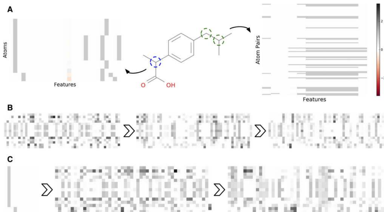
Fig. 8. Graph convolution feature evolution. Atoms or pairs are displayed on the y -axis and the dimensions of the feature vectors are on the x -axis. a Conversion of the molecular graph for ibuprofen into atom and (unique) atom pair features. b Evolution of atom features after successive Weave modules in a graph convolution model with a W_3N_2 architecture and depth 50 convolutions in Weave modules. c Evolution of “simple” atom features (see “Input featurization” section) starting from initial encoding and progressing through the Weave modules of a W_2N_2 architecture. The color bar applies to all panels
