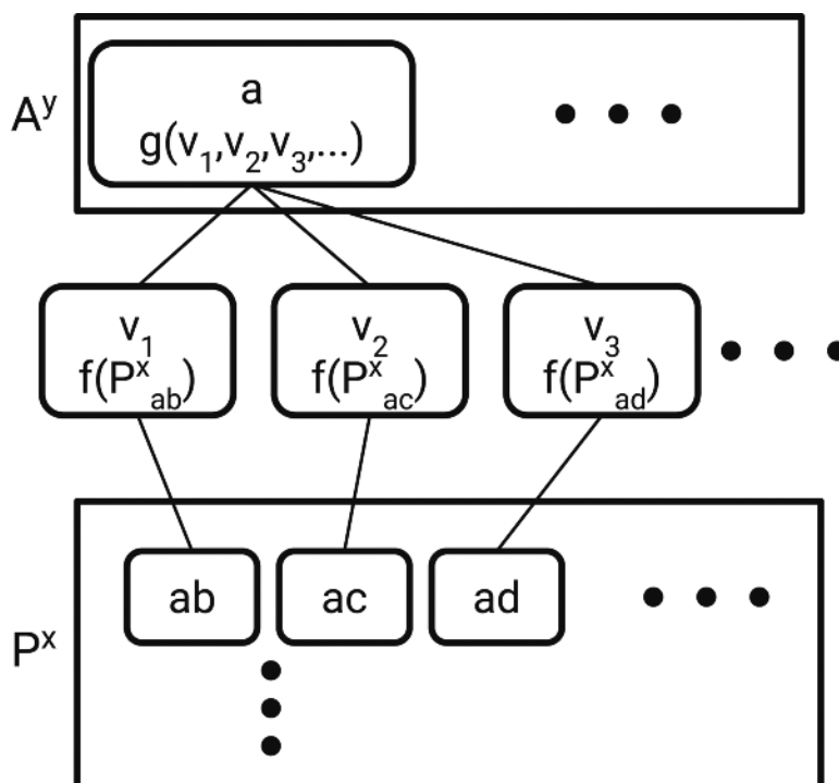
Fig. 2. P \rightarrow A operation. P^x is a matrix containing features for atom pairs ab , ac , ad , etc. The v_i are intermediate values obtained by applying f to features for a given atom pair. Applying g to the intermediate representations for all atom pairs involving a given atom (e.g. a ) results in a new atom feature vector for that atom
