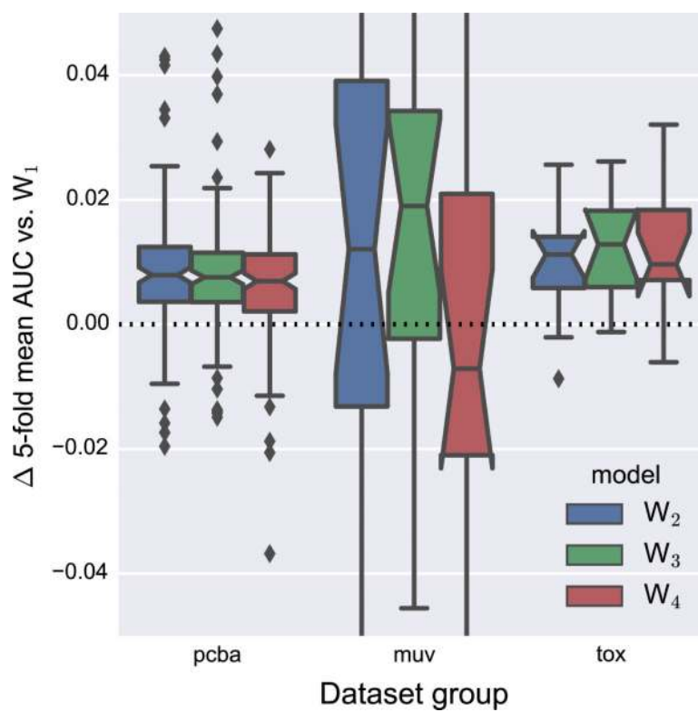
Fig. 9. Comparison of models with different numbers of Weave modules with a model containing a single Weave module. All models used a maximum atom pair distance of two. The y-axis is cropped to emphasize differences near zero
