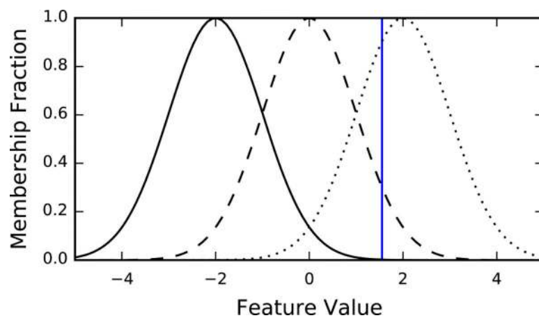
Fig. 5. Fuzzy histogram with three Gaussian “bins”. Each curve represents the membership function for a different bin, indicating the degree to which a point contributes to that bin. The vertical blue line represents an example point which contributes normalized densities of <0:01 , \sim 0:25 , and \sim 0:75 to the bins (from left to right )
