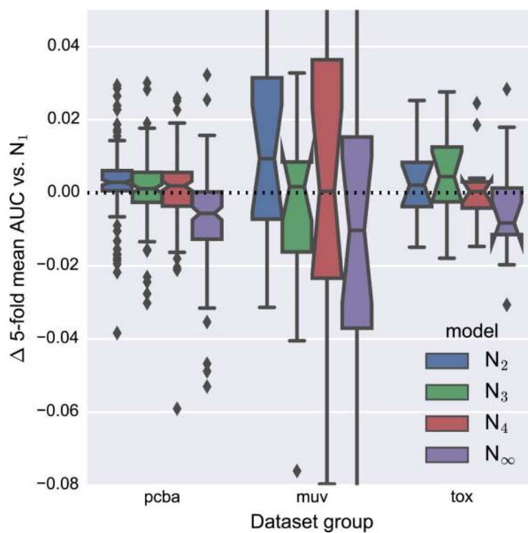
Fig. 11. Comparison of models with different maximum atom pair distances to a model with a maximum pair distance of one (bonded atoms). All models have two Weave modules. The y -axis is cropped to emphasize differences near zero
