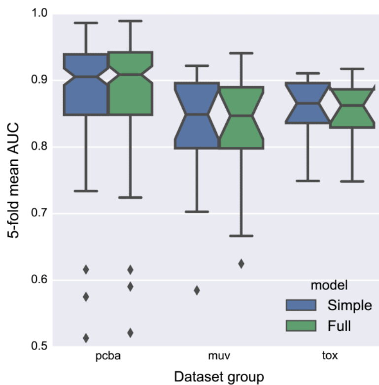
Fig. 7. Comparison of models with “simple” and “full” input featurizations. The simple featurization only encodes atom type, bond type, and graph distance. The full featurization includes additional features such as aromaticity and hydrogen bonding propensity (see “Molecule-level features” section for more details). Confidence intervals for box plot medians were computed as \pm 1.57 \times IQR / \sqrt{N} [20]
