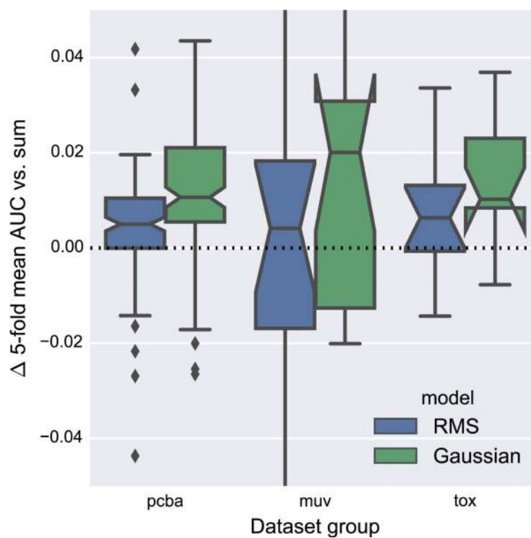
Fig. 10. Comparison of root-mean-square (RMS) and Gaussian histogram reductions versus sum reduction. The y -axis reports difference in fivefold mean AUC relative to sum reduction. All models used two Weave modules and a maximum atom pair distance of two. The y -axis is cropped to emphasize differences near zero
