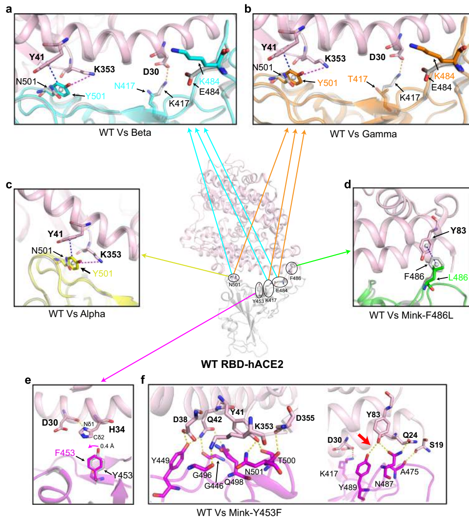
Fig. 3 Structural comparison of WT RBD-hACE2 and each SARS-CoV-2 variants RBD-hACE2. a–e The WT RBD-hACE2 structure (PDB: 6LZG) is shown in the center. Superimposition of WT RBD-hACE2 and each variant RBD-hACE2 (including Beta RBD-hACE2 ( a ), Gamma RBD-hACE2 ( b ), Alpha RBD-hACE2 ( c ), Mink-F486L RBD-hACE2 ( d ), Mink-Y453F RBD-hACE2 ( e )) are shown in each surrounding panel. In each structure the hACE2 is colored in light pink. SARS-CoV-2 WT RBD, Beta RBD, Gamma RBD, Alpha RBD, Mink-F486L RBD, and Mink-Y453F RBD are colored in gray, cyan, orange, yellow, green, and magenta, respectively. The key contact residues are shown as stick structures and labeled appropriately. The cation- \pi interaction, \pi - \pi stacking interaction, salt bridge, and hydrogen bonds are colored in magenta, blue, orange, and yellow, respectively. Hydrogen bond interactions were analyzed at a cutoff of 3.5 Å. f The detailed hydrogen bonds between the Mink-Y453F RBD and hACE2 are shown.
