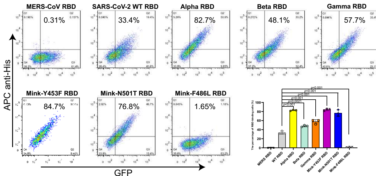
Fig. 1 Characterization of binding between different RBDs and hACE2 using flow cytometry. BHK cells stably expressing GFP and hACE2 were incubated with His-tagged MERS-CoV RBD, SARS-CoV-2 WT RBD, Alpha RBD, Beta RBD, Gamma RBD, Mink-Y453F RBD, Mink-N501T RBD, and Mink-F486L RBD, respectively. APC anti-His antibodies were used to detect the His-tagged protein binding to the cells. Representative results from three experiments are shown. The mean \pm SD percentages of RBD-binding cells in the three experiments are shown in the right lower bar chart. Statistical significance was analyzed using one-way ANOVA with a Tukey's multiple comparison test for multiple groups.
