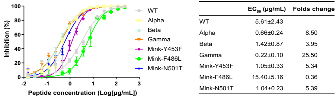
Fig. 5 Neutralization of SARS-CoV-2 variants by hACE2. The EC 50 values and folds change values are shown on the right panel. The folds change was normalized to WT, and the EC 50 values are presented as the mean ± SEM of three independent replicates ( n = 3 ). The representative results from three experiments are shown.
