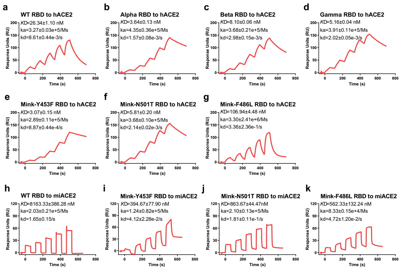
Fig. 2 Binding affinity of SARS-CoV-2 RBDs to ACE2, characterized by SPR. a–k Mouse Fc (mFc)-fused hACE2 or miACE2 in the supernatant was captured in the CM5 chip via its interaction with the pre-immobilized anti-mFc antibody. Various concentrations of SARS-CoV-2 WT RBD ( a ), Alpha RBD ( b ), Beta RBD ( c ), Gamma RBD ( d ), Mink-Y453F RBD ( e ), Mink-N501T RBD ( f ), and Mink-F486L RBD ( g ) protein were used to evaluate their binding affinity for hACE2. Serially diluted WT RBD ( h ), Mink-Y453F RBD ( i ), Mink-N501T RBD ( j ), and Mink-F486L RBD ( k ) protein were measured the binding to miACE2. K_D , k_a , and k_d values are all recorded and the representative results from three experiments are shown. The data are presented as the mean \pm SEM of three independent replicates ( n = 3 ).
