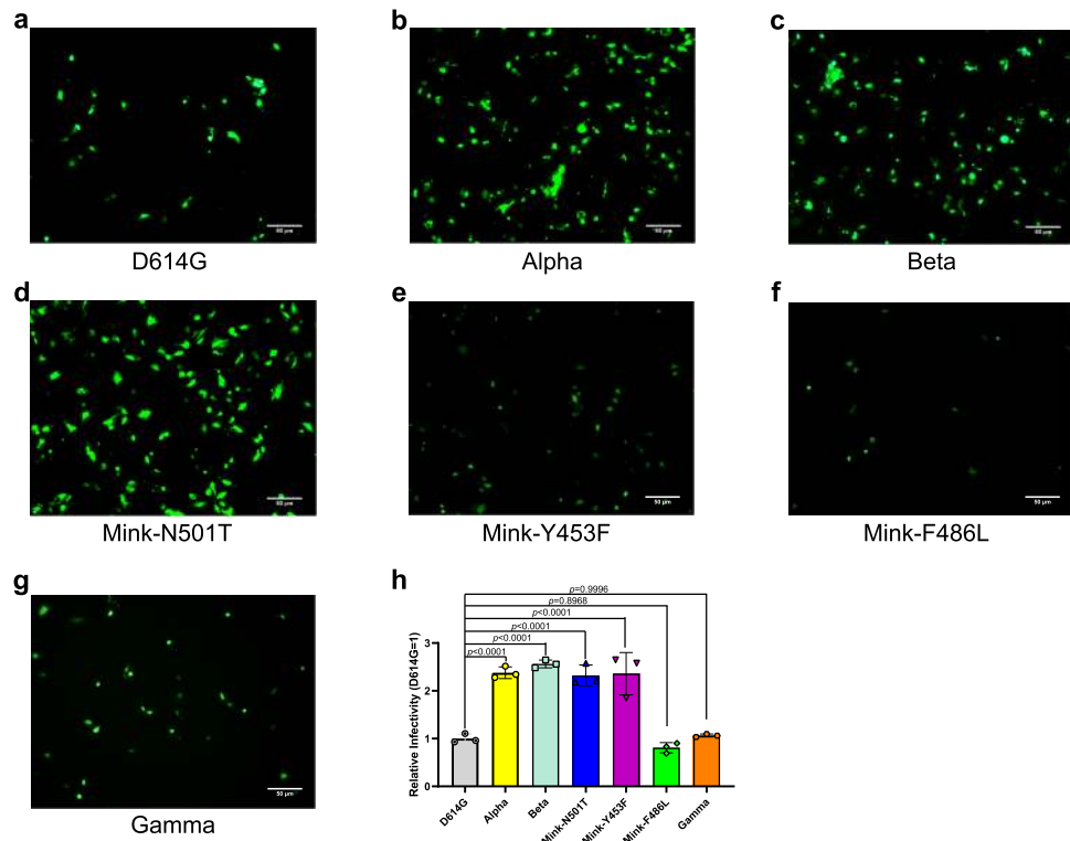
Fig. 4 Entry of SARS-CoV-2 variant pseudoviruses into Huh7 cells. a–g The SARS-CoV-2 D614G ( a ), Alpha ( b ), Beta ( c ), Mink-N501T ( d ), Mink-Y453F ( e ), Mink-F486L ( f ), and Gamma ( g ) pseudoviruses' entry into Huh7 cells as evidenced by GFP expression in transduced cells. The representative results from three experiments are shown. h The GFP-positive cells were quantified using FACS and representative results from three experiments are shown. The values indicate the mean of the three experiments and the bar suggest the SD. Relative infectivity was normalized against that of the D614G pseudovirus. Statistical significance was analyzed using a one-way ANOVA with Tukey's multiple comparison test for multiple groups.
