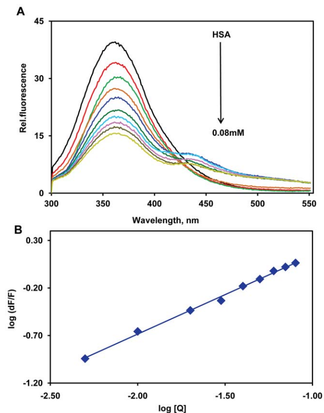
Figure 2. Fluorescence emission spectra of HSA-TMF in 0.1 M phosphate buffer pH 7.2, \lambda_{ex} = 285 nm, temperature = 25 \pm 1^\circ\text{C} . A) Free HSA (0.025 mM) and free HSA with different concentrations of TMF (0.005, 0.01, 0.02, 0.03, 0.04, 0.05, 0.06, 0.07, 0.08 mM). B) Plot of \log(dF/F) against \log[Q] . \lambda_{ex} = 285 nm \lambda_{em} = 362 nm. doi:10.1371/journal.pone.0008834.g002
