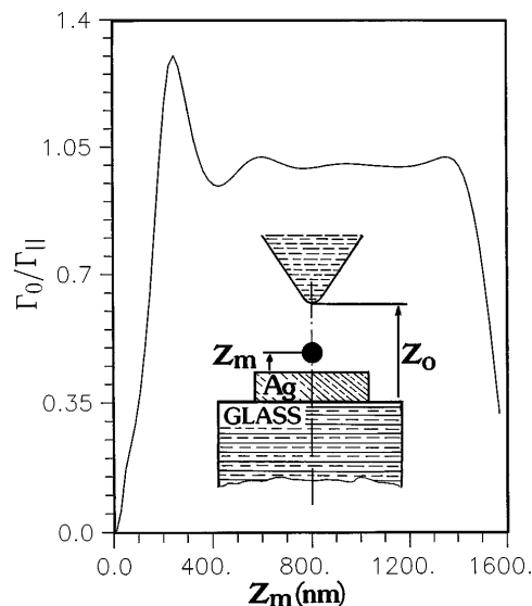
FIG. 2. Distance dependence of the normalized lifetime \Gamma_0/\Gamma_{\parallel} inside the junction, as a function of the position of the molecule. The geometry used in the simulation is described in the inset and the tip-sample separation is maintained at Z_0 = 1600 nm. The glass sample is covered with a square shaped silver layer 300 nm long and 20 nm high.
