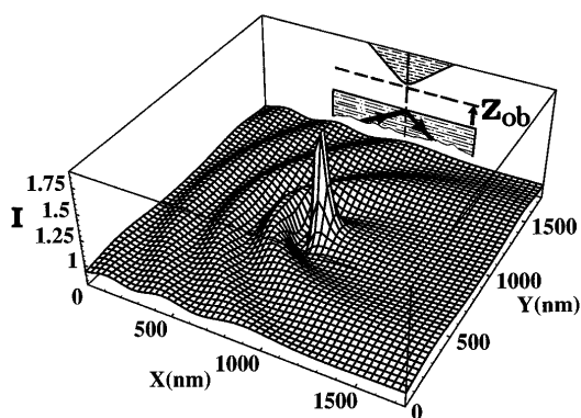
FIG. 1. Illustration of scattering and light confinement in the vicinity of a SNOM junction [14]. The three-dimensional map represents the normalized field intensity I = |E|^2/|E_0|^2 , calculated in the observation plane Z_{\text{obs}} = 20 nm. The tip-sample distance is 30 nm and the system is illuminated in internal reflection in the p -polarized mode. The optical indexes of tip and sample are identical ( n = 1.5 ) and the incident wavelength \lambda = 600 nm. In the present configuration, the FWHM of the peak reaches about 75 nm.
