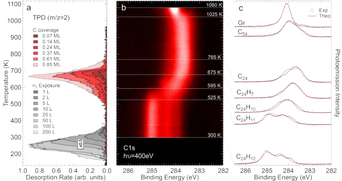
Figure 3: (a) Temperature programmed desorption spectra (red scale) of m/z = 2 after coronene deposition at different coverage and T = 300 K. For comparison desorption spectra (grey scale) corresponding to m/z = 2 after molecular hydrogen adsorption at T = 100 K are reported (intensity rescaled by a factor 0.5). (b) Temperature dependent C 1s core level spectra (about 100 spectra) shown as a two-dimensional intensity plot. (c) Comparison between selected experimental C 1s core-level spectra and fit results (red curves).
