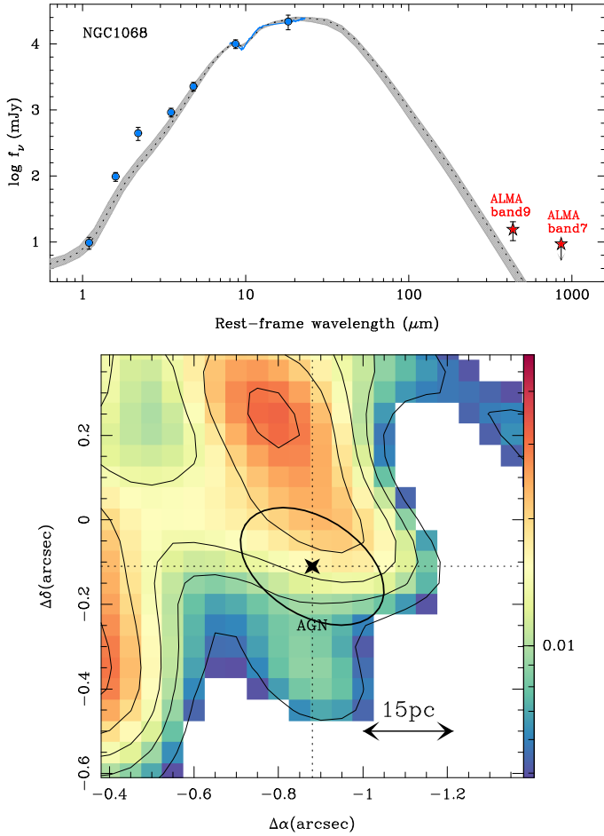
Fig. 3. Upper panel: the nuclear SED of the dust continuum emission in NGC 1068 derived using NIR and MIR continuum and spectroscopy data (blue squares) from Alonso-Herrero et al. (2011), and the ALMA data points in Bands 7 and 9 (red stars). The SED was derived in apertures centered at the AGN that range from 0''.2 ( \sim 14 pc) for NIR data to 0''.5 ( \sim 35 pc) for MIR and Band-7 ALMA data. The best CLUMPY model fit to the observations (curve) and the 1\sigma uncertainty range of the fit (gray shaded region) are superposed onto the data points. Lower panel: a close-up view of the dust continuum emission in Band 9. Levels and markers are as in Fig. 1. The (0''.4 \times 0''.2) -aperture used to extract the flux at the position of the AGN is plotted as an ellipse.
