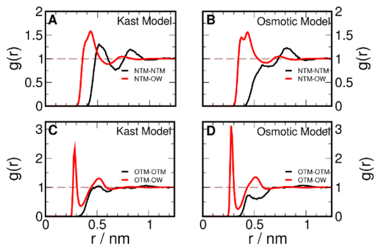
Figure 2. Radial distribution functions in 2 molal TMAO solution. Distributions of TMAO nitrogen (NTM) and water oxygen (OW) around TMAO nitrogen shown for (A) Kast Model and (B) Osmotic Model. Distributions of TMAO oxygen (OTM) and water oxygen (OW) around TMAO oxygen shown for (C) Kast Model and (D) Osmotic Model.
