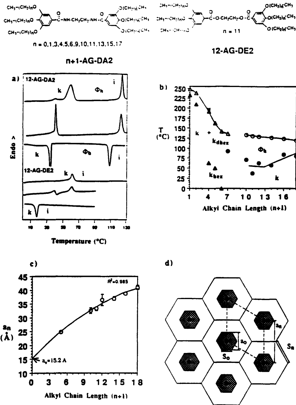
FIGURE 12: (a) DSC traces from the first heating scan, second heating scan, and first cooling scan (top to bottom) for 12-AG-DA2 and 12-AG-DE2; (b) the phase behavior of n+1-AG-DA2 versus alkyl tail length (n+1); (c) extrapolation of the experimentally measured column radius ( a_n ) determined from x-ray scattering experiments in the k_{\text{hex}} of \Phi_h phases versus alkyl tail length; (d) illustrative definitions of a_n , a_0 , S_n , and S_0 for the hexagonal columnar phase.
