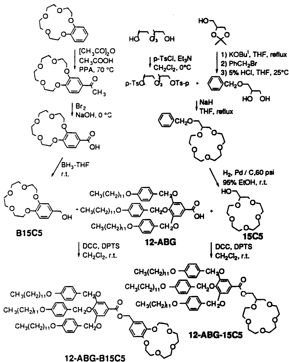
FIGURE 3: Synthesis of 12-ABG-B15C5 and 12-ABG-15C5 building blocks. (PPA = polyphosphoric acid; p-TsCl = p-toluenesulfonyl chloride; THF = tetrahydrofuran; DDC = dicyclohexycarbodiimide; DPTS = N,N-dimethylaminopyridinium p-toluenesulfonate)
