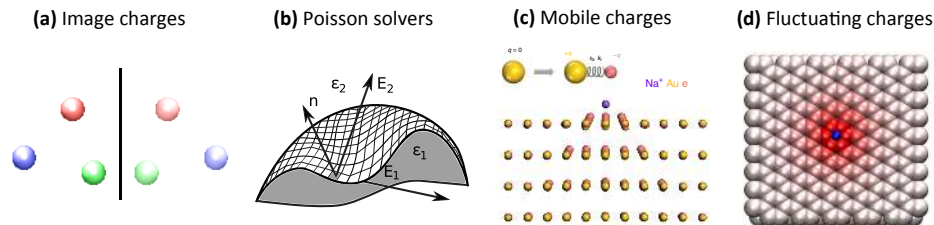
FIG. 1: Strategies to account for the polarization of the metal by the electrolyte in molecular simulations. (a) Image charges q^{im} inside the solid with permittivity \epsilon_2 induced by the electrolyte charges q^{ext} in a medium of permittivity \epsilon_1 (see Eq. 1). (b) Solving the Poisson equation on a grid to compute the induced (surface) charges. (c) Describing the electronic response with mobile charges: here gold atoms are modeled using opposite charges tethered by a spring, with the cores representing the nuclei (yellow) fixed and the shells (pink) moving in response to the presence of a sodium ion (purple). (d) Describing the electronic response with fixed sites with fluctuating charges: here the charge of atoms in a graphite electrode is distributed inhomogeneously (darker red means more negative) in response to the presence of a cation such as \text{Li}^+ (blue). Panel b reproduced from Ref. [42], J. Chem. Phys. 2010, 132 , 154112, with the permission of AIP Publishing; panel c reproduced from Ref. [45], Nature Commun. 2018, 9 , 716, with permission of Springer Nature.
