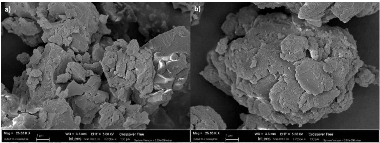
Figure 7. FESEM images of a) NIP(1:4) and b) MIP(1:4)+10%L-DOPA. Magnification 25 K.
