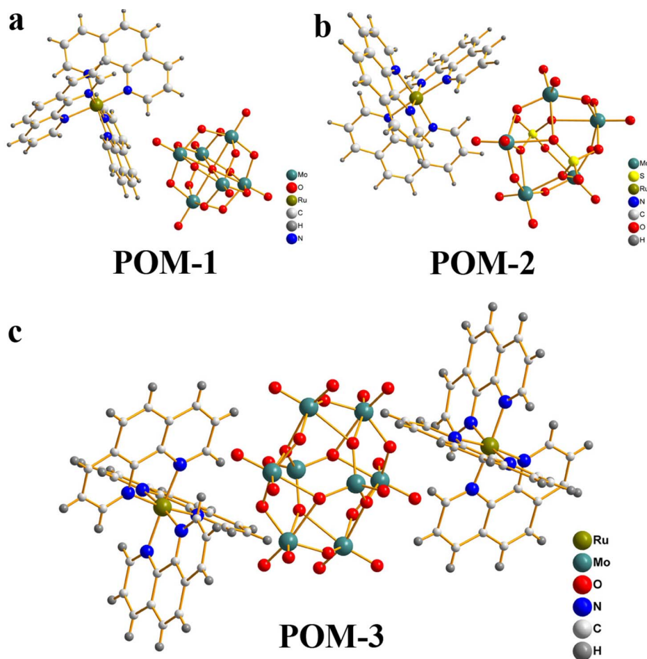
Figure 1 | The structures of hybrid materials POM-1–3.
