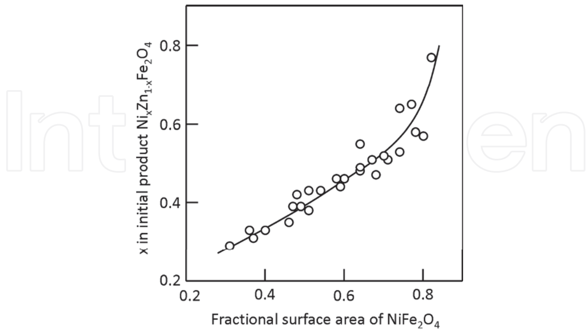
Fig. 9. The relative surface area of \text{NiFe}_2\text{O}_4 particles determines the Ni concentration in (\text{Ni,Zn})\text{Fe}_2\text{O}_4 (Hayashi et al., 1985).
