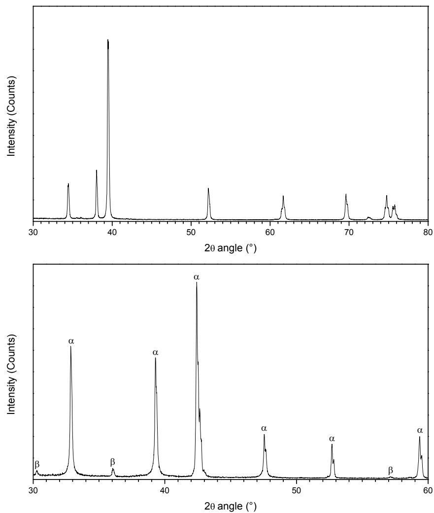
Figure S1. XRD patterns of Mo 2 C (top) and MoB (bottom). For MoB, the assignments of the alpha ( \alpha ) and beta ( \beta ) phases are shown.
