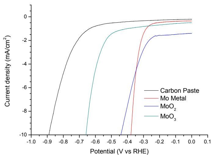
Figure S11. Polarization curves of MoO 2 , MoO 3 , Mo, and carbon paste electrodes. (Top)
