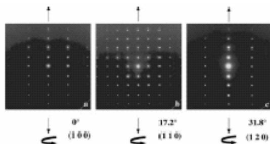
Fig. 2. Tilting series of diffraction patterns taken from an isolated small single crystal. The correct Miller indices are given for each pattern after crystallographic analysis.
