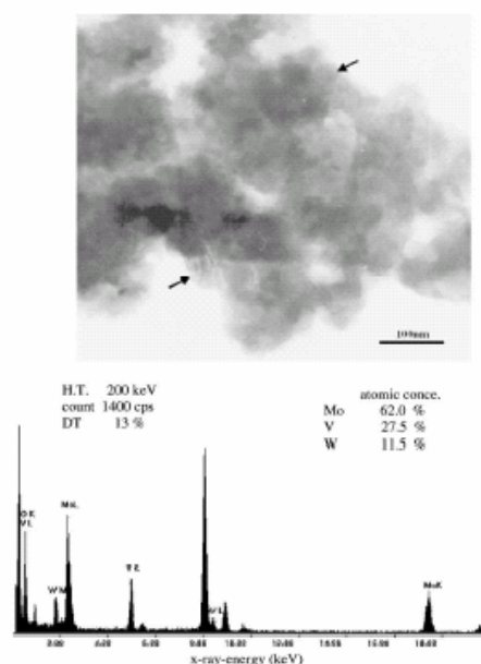
Fig. 1. Electron micrograph of the mixed oxide catalyst taken with objective aperture in order to enhance the contrast of crystallized particles. The sharp boundaries of crystallized particles are indicated by arrows. The EDX spectrum was taken from an isolated crystallized particle.
