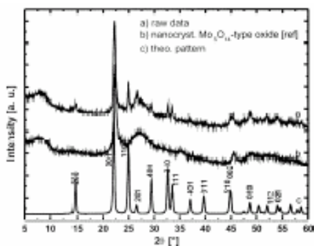
Fig. 5. XRD pattern of the MoVW mixed oxide operated in the acrolein oxidation (diffractogram a); reference XRD pattern of the nanocrystalline MoVW oxide prior to catalysis (diffractogram b) [1 and 2], XRD pattern simulated from the estimated space group and atomic positions (diffractogram c).
