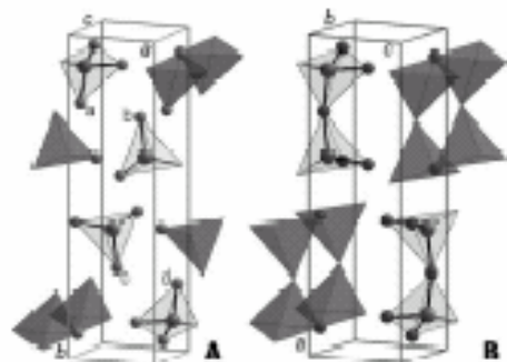
Fig. 6. (A) A schematic picture of atomic configuration in a unit cell of \text{MoO}_3 . The oxygen–oxygen weak binding positions are indicated between a and b , and c and d ; (B) a schematic picture of atomic configuration in a unit cell of the alternative crystal model. This crystal has been constructed through the two successive sliding operations at a – b and c – d , as described in the text.
