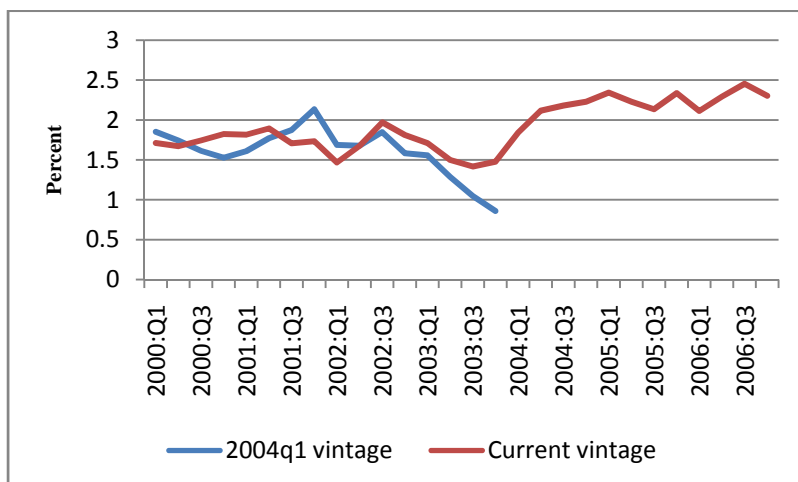
Figure 3: Real-Time and Revised Core PCE Inflation
