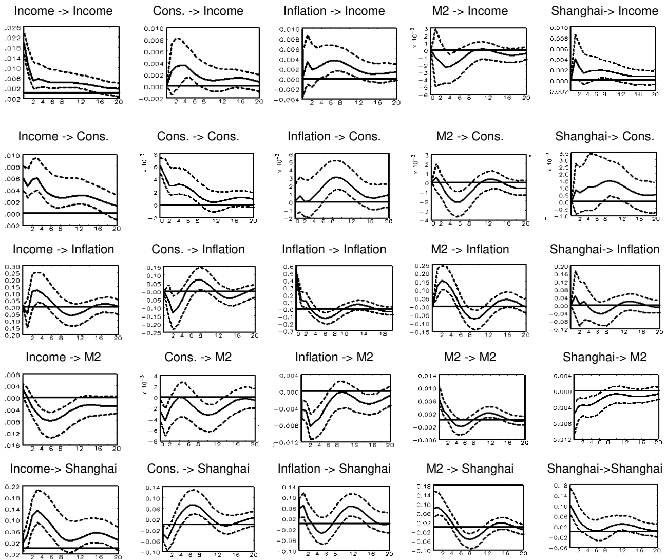
Figure A3. Impulse response analysis with Shanghai A-Index.
