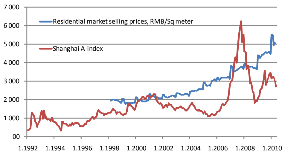
Figure 1. Shanghai A-Index and residential prices in China.
