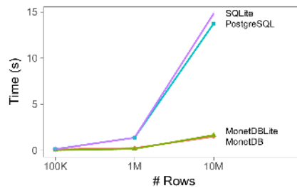
(b) Run TPC-H Q1 inside the database.
