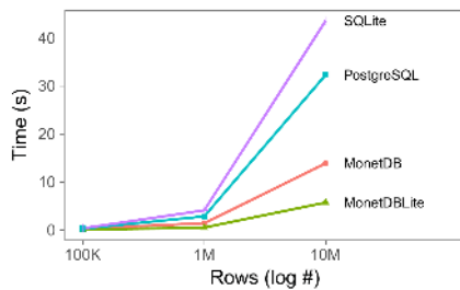
(a) Transfer data from database to client.
