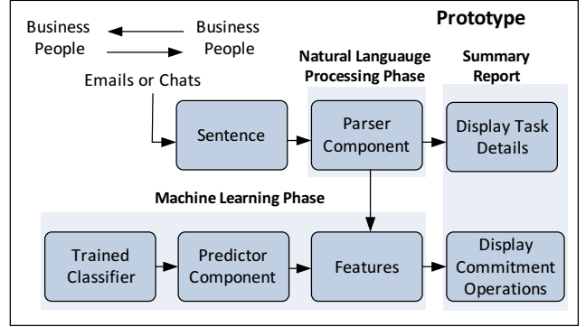
Fig. 10. The architecture of our commitment identification and monitoring tool.
