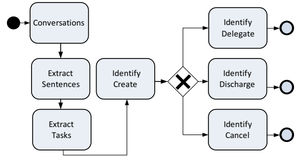
Fig. 3. Process followed to identify commitments.
