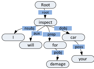
Fig. 4. Typed dependencies derived from a sentence “I will inspect your car for damage” in Table I.
