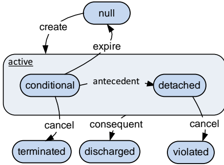
Fig. 2. The lifecycle of a commitment [3].
