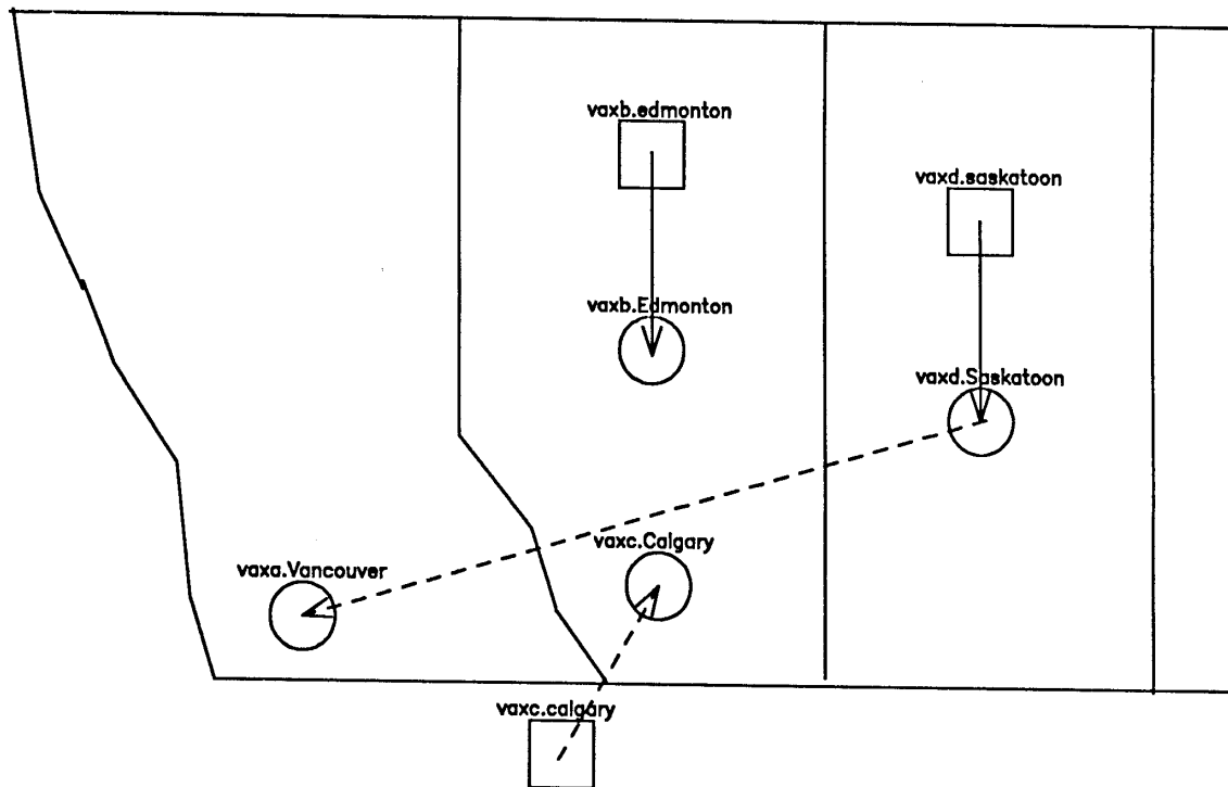
Figure 3.3: Mona Frame of the Distributed Banking System
