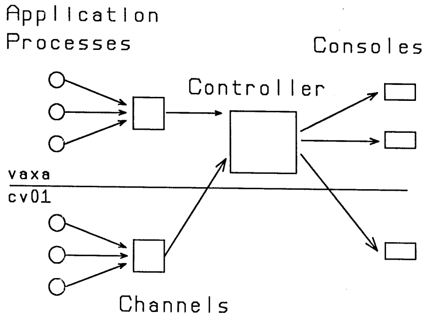
Figure 2.5: The Monitoring System with Controller
