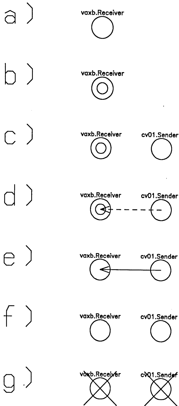
Figure 3.2: Graphical Frames Corresponding to Textual Trace
