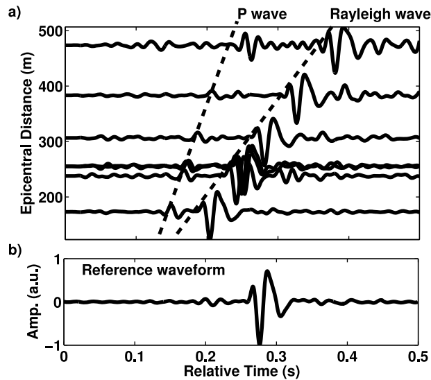
Figure 3. (a) Amplitude normalized vertical-component waveforms at stations BG1 through BG7 for the event shown in Figure 2. The waveforms are plotted as a function of epicentral distance; however, t = 0 does not correspond to the origin time. (b) The reference waveform is generated by aligning all waveforms in Figure 3a on the Rayleigh wave and summing. This suppresses the P wave and background noise.
