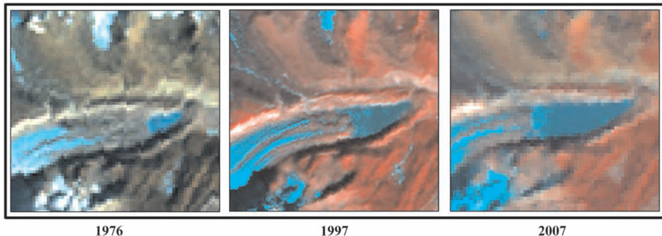
Figure 14: Changes in Lonak lake, Tista basin, Sikkim, India between 1976 and 2007.
