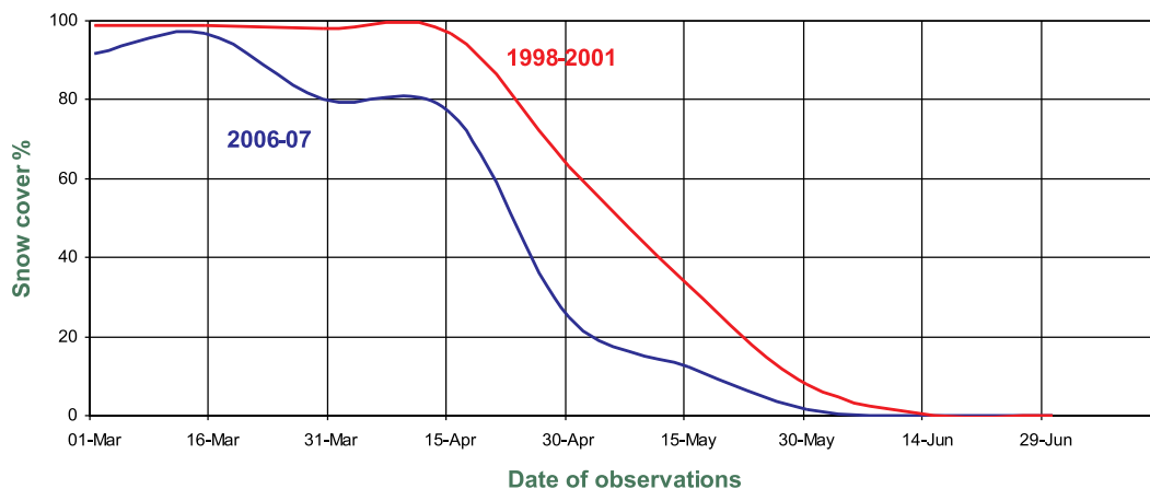
Figure 8: Snow cover depletion curve for altitude 3000–3600 m in the Beas basin, India.
