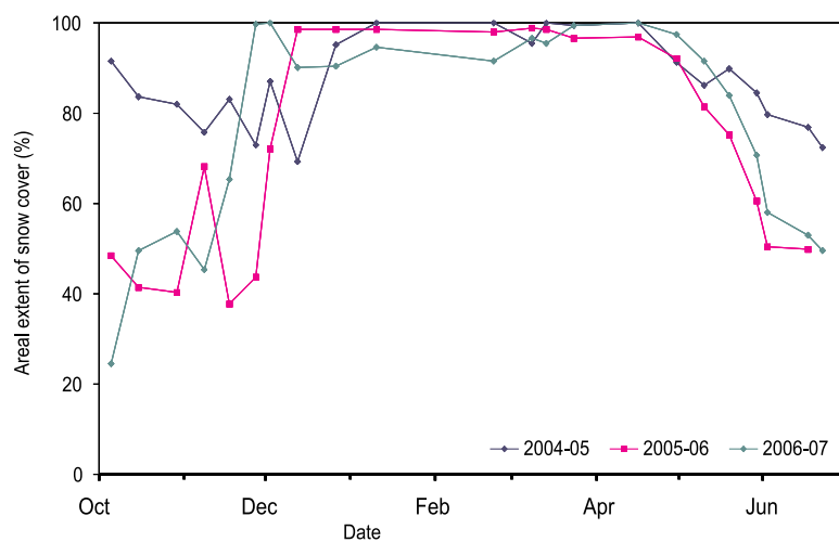
Figure 9: Snow accumulation and ablation curve of Bhaga basin.
