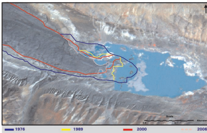
Figure 2: Satellite imagery of IRS LISS-IV sensor of September 16, 2006 showing retreat of Samudra Tapu glacier, Himachal Pradesh, India from 1976.
