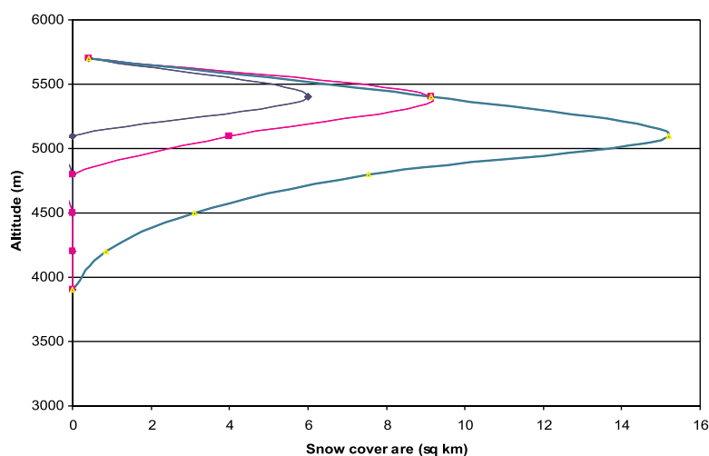
Figure 13: Changes in accumulation area of glacier due to rise in temperature by 1°C. Red line suggest present and blue line suggest future distribution of Accumulation area.
