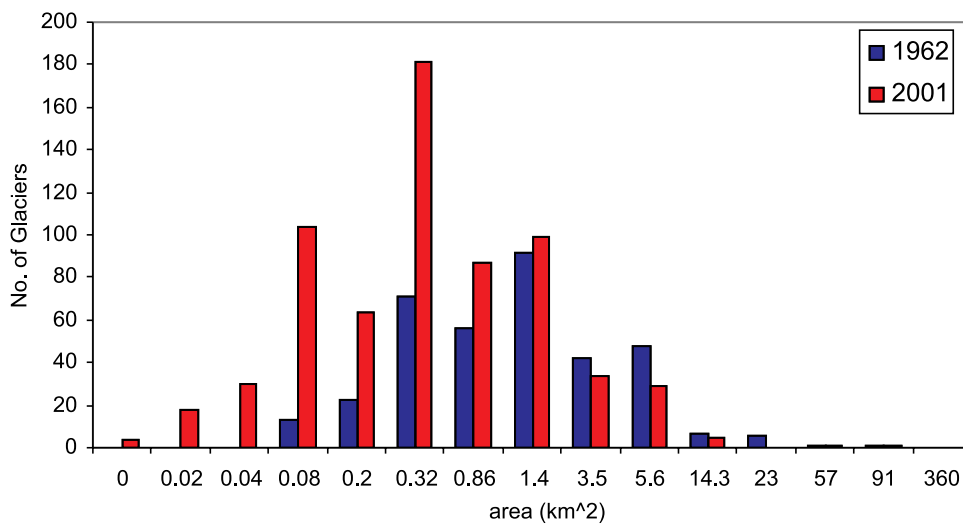
Figure 4: Number of glaciers as a function of area for Chenab basin. Areal extent in bin increases by power of 2.
