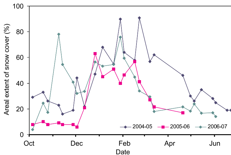
Figure 10: Snow accumulation and ablation curve of Ravi basin.
