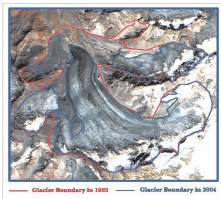
Figure 5: Resourcesat imagery of LISS-IV sensor dated September 12, 2004 of glacier number 52E09027. The glacier is split into 4 glaciers between 1962 and 2004. However areal extent is reduced from 7.0 to 5.3 km 2 .
