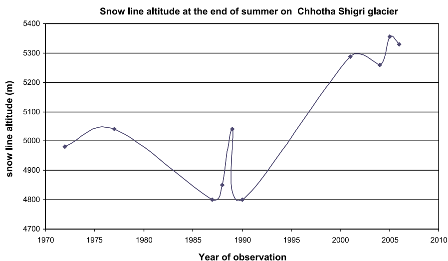
Figure 6: Snow line altitude at the end of ablation season on Chhota Shigri glacier, Himachal Pradesh.
