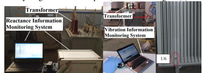
(a) Reactance test site (b) Vibration test site (c) Vibration test point
