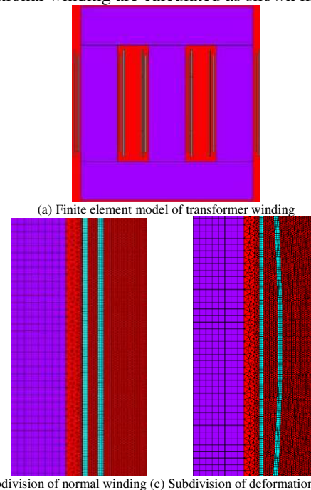
(a) Finite element model of transformer winding (b) Subdivision of normal winding (c) Subdivision of deformational winding FIGURE 10. Finite element simulation model of transformer winding
