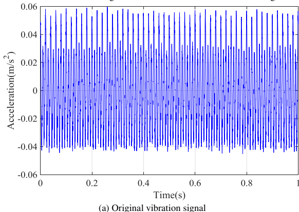
FIGURE 18. Vibration signal and CEEMD result in normal winding state
