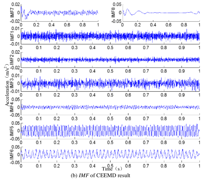
FIGURE 19. Vibration signal and CEEMD result of winding after short circuit current impacts
