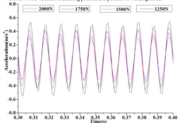
FIGURE 8. Vibration calculation results in different compression forces
