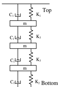
FIGURE 2. The winding mechanical kinetic model
