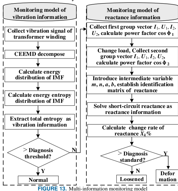
FIGURE 13. Multi-information monitoring model
