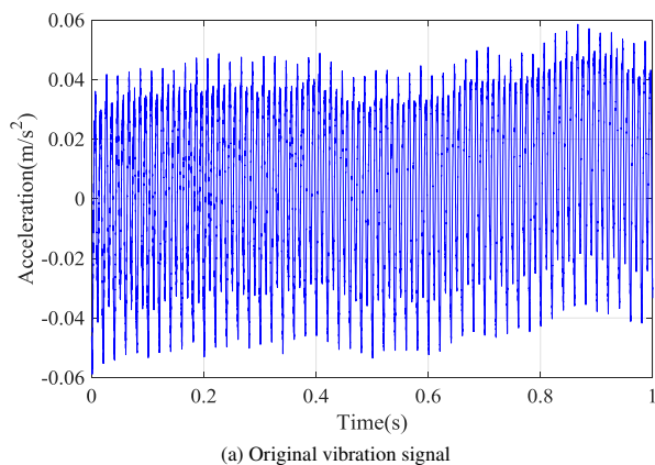
FIGURE 22. Vibration signal and CEEMD result in deformational winding of axial tension loosened
