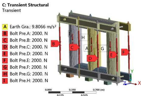
FIGURE 6. Compression force on winding vibration model
