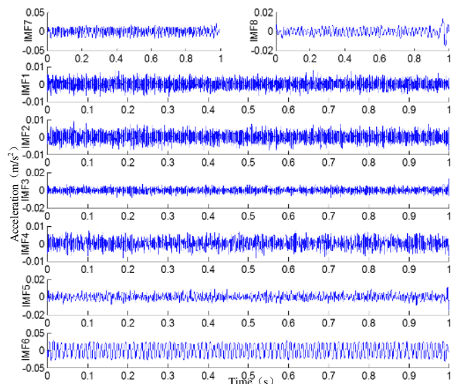
FIGURE 23. Vibration signal and CEEMD result in deformational winding of coil folding in end position
