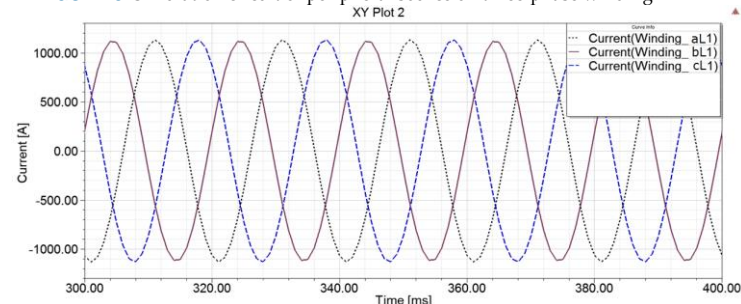
(a) Load currents of low-voltage windings
