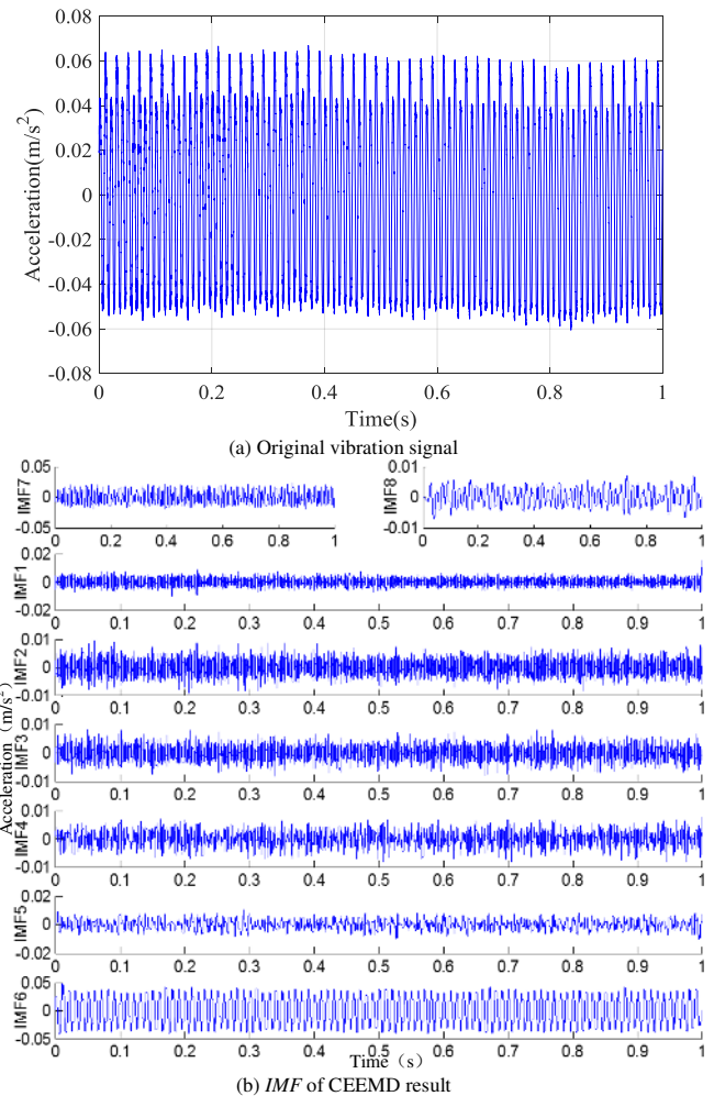
FIGURE 21. Vibration signal and CEEMD result in deformational winding of radial extension in the middle position
