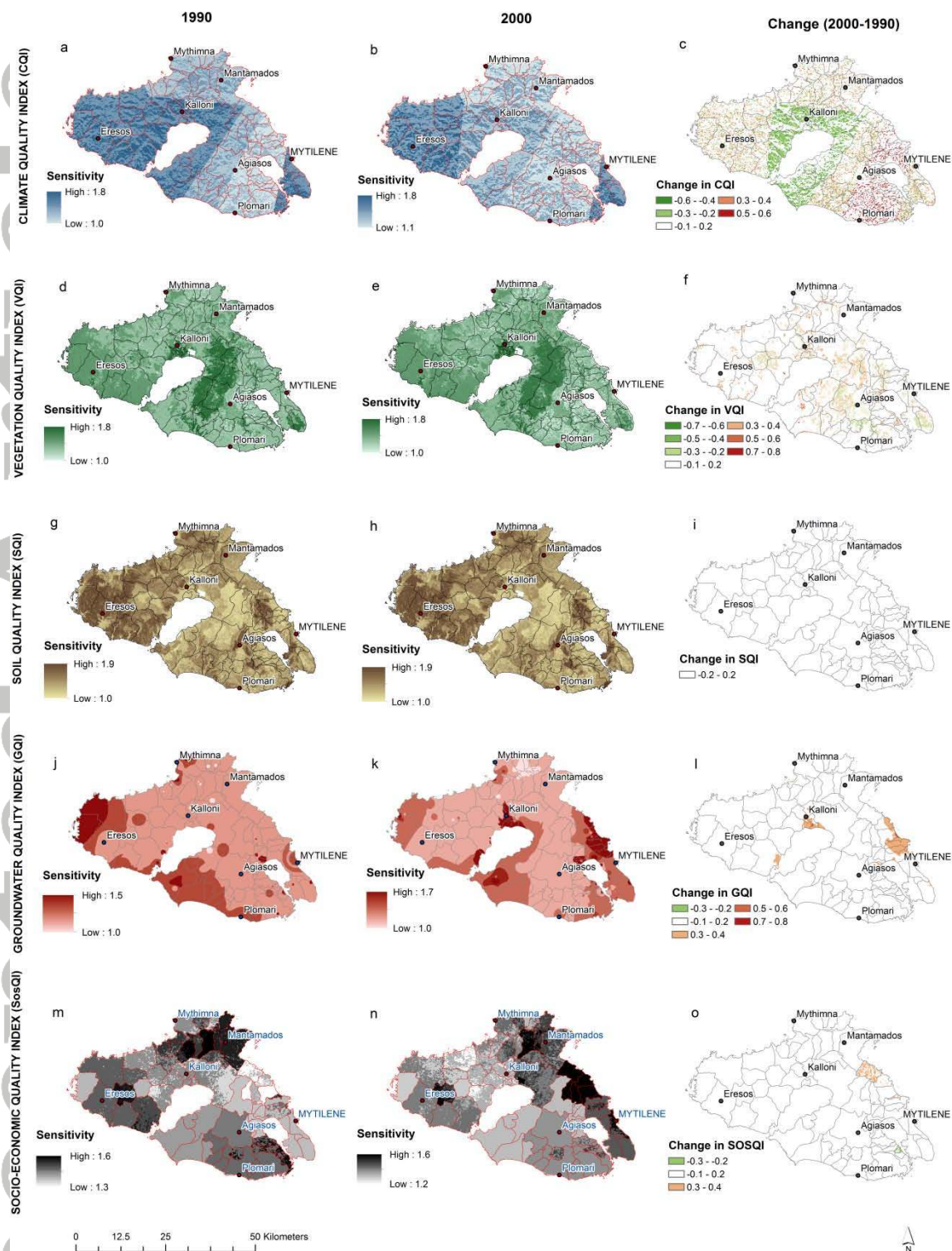
Figure 3. Sensitivity maps for 1990 and 2000 and respective change: (a), (b), (c) Climate Quality Index (CQI); (d), (e), (f) Vegetation Quality Index (VQI); (g), (h), (i) Soil Quality Index (SQI); (j), (k), (l) Groundwater Quality Index (GQI); (m), (n), (o) Socioeconomic Quality Index (SosQI).
