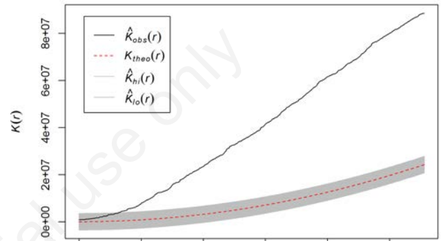
Figure 8. Ripley's K function [K(r)] vs distance (r) for adopted dogs and cats. Confidence envelopes (grey band) include the upper and the lower limit of the K_{theo}(r) (red line) showing a clustered pattern at different distances compared to the K_{obs}(r) (black line) after 99 simulations ( P=0.01 ).
