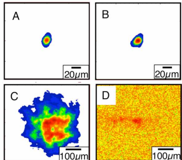
FIGURE 2. Mode images of laser propagation at 4 TW. The output image with the guide on (b) is indistinguishable from the input (a) indicating unaberrated propagation at twice P crit . Unguided images show diffraction in vacuum (c) and ionization enhanced diffraction with the gas jet on (d).
