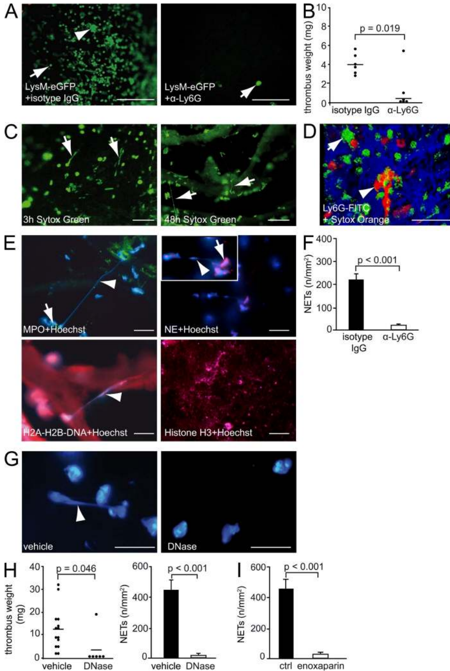
Figure 6. NETs propagate DVT in vivo. (A) Leukocyte accumulation in vivo at 6 h of flow restriction in the IVC of LysM-eGFP mice treated with control antibody or the anti-Ly6G mAb to deplete neutrophils. Arrowhead: aggregated neutrophils; arrows: single, adherent cells. Bars, 100 \mu m. (B) Thrombus weight 48 h after DVT induction in isotype and anti-Ly6G-treated WT mice ( n = 6 per group). Dots represent individual experiments; lines show the mean of each group. (C) Representative image of n = 3 experiments of intravital microscopy 3 or 48 h after flow reduction showing Sytox Green + NETs in the IVC. Bars, 50 \mu m. (D) Visualization of NETs in vivo by 2-photon microscopy. Ly6G-positive neutrophils (green, FITC anti-Ly6G antibody) attached to the vessel wall (blue) release Sytox orange-positive (red) NET structures inside the IVC 4 h after flow reduction (also see Video 7). Sytox orange-positive nuclei correspond to dying neutrophils, which have not (yet) exposed their DNA to the extracellular space. Arrowhead: extracellular DNA; arrow: neutrophil. Bar, 50 \mu m. (E) Immunohistochemical visualization of NETs by staining for DNA (Hoechst), MPO, NE, and histones (H2A-H2B-DNA, H3) in the IVC of WT mice 48 h after induction of DVT. Hoechst + DNA originating from MPO + NE + neutrophils (arrows) could be detected. Arrows, nuclei; arrowheads, NET fibers. Bars, 10 \mu m. (F) Number of NETs in neutropenic mice were quantified in thrombi after treatment with anti-Ly6G and isotype control antibody ( n = 3 per group). Data are shown as mean \pm SEM. (G) Representative images of WT thrombi stained with Hoechst after DNase1 treatment. Arrowhead, NET fiber. Bars, 10 \mu m. Shown is a representative of n = 3 experiments. (H) After injection of DNase1, thrombus weight (left) in the IVC was determined after 48 h of flow restriction. Dots represent individual experiments; lines show the mean of each group. Quantification of NETs is also shown (right) as mean \pm SEM. Data were obtained in WT injected with normal saline i.v. ( n = 14 ) or DNase1 ( n = 6 ). (I) Quantification of NETs at 48 h in the enoxaparin-treated animals ( n = 4 per group). Data are shown as mean \pm SEM.
