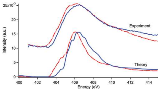
Figure 2. Measured nitrogen K-shell NEXAFS spectra of alanine and sarcosine and the computed spectra aligned to experiment are shown above. For both experiment and theory, sarcosine (blue) is shifted slightly to higher energy than alanine (red and dashed); the slight shift is reproduced well in the computed spectra and is assigned primarily to methyl group substitution on the nitrogen in sarcosine.
