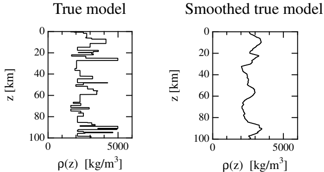
Figure 5: The true model used to generate synthetic data.
