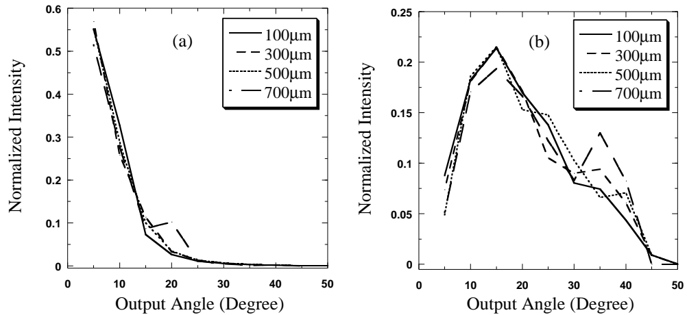
Figure 6. Normalized angular distributions of (a) the Class I signal and (b) the Class II signal for various probing depths, where r_d = 10 \mu\text{m} and the other simulation parameters are the same as those in figure 3.
