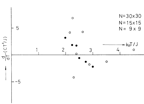
Fig. 11. Temperature derivative of energy correlation for the two-dimensional XY-model.
