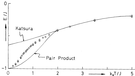
Fig. 3. Temperature-dependence of the total energy for the one-dimensional quantum XY-model ( N=33, n=2 ); “Pair Product” means the analytic solution for N=\infty, n=1 , and “Katsura” means the rigorous solution of this model.
