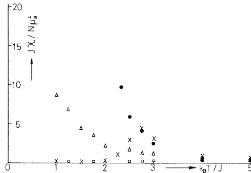
Fig. 13. Temperature-dependence of susceptibility for two-dimensional models; “●”, XY-model (15×15); “△”, Heisenberg model; “×”, Ising model and “□”, \chi_{II} in the XY-model.
