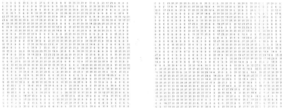
Fig. 14. Typical spin configurations of the effective lattice: (a) k_B T = 3.0J , (b) k_B T = 2.25J , where each number in the figures represents states of five Ising spins corresponding to each real spin in the binary system: 0 = (\downarrow, \downarrow, \downarrow, \downarrow, \downarrow) , 31 = (\uparrow, \uparrow, \uparrow, \uparrow, \uparrow) or 12 = (\downarrow, \uparrow, \uparrow, \downarrow, \downarrow) . M_1 denotes the number of up spins in the real space.
