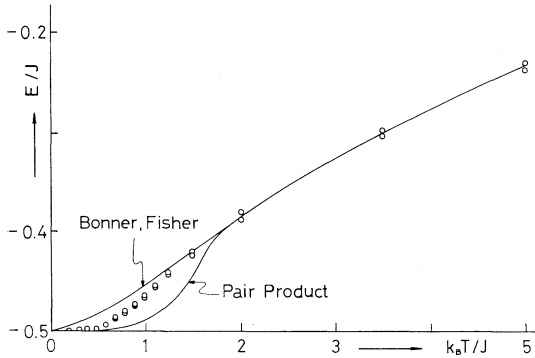
Fig. 5. Temperature-dependence of the total energy for the one-dimensional quantum Heisenberg model ( N=33, n=2 ); “Bonner, Fisher” means an extrapolation from exact numerical solutions in finite systems.
