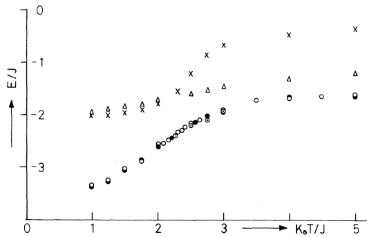
Fig. 8. Temperature-dependence of the energy for the two-dimensional models; “x”, Ising model (9×9); “Δ”, Heisenberg model (9×9); “●”, XY-model (9×9); “○”, XY-model (15×15) and “⊙”, XY-model (30×30).
