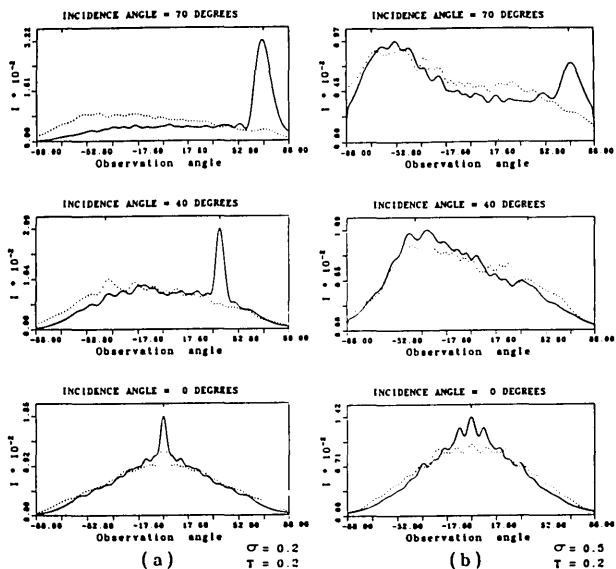
Fig. 1. Mean scattered intensity for (a) T = 0.2\lambda , \sigma = 0.2\lambda , (b) T = 0.2\lambda , \sigma = 0.5\lambda , and several angles of incidence. Solid curves, s waves; dotted curves, p waves.
