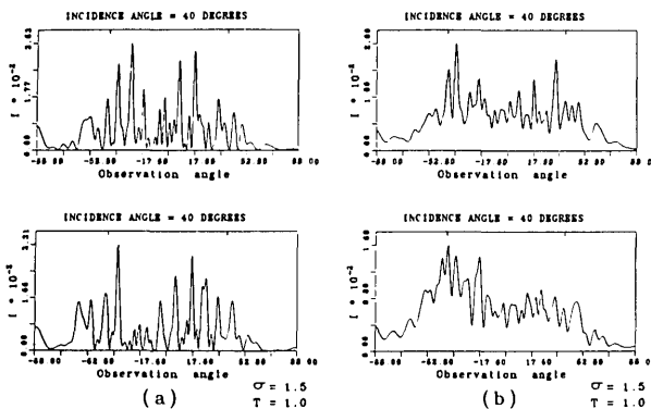
Fig. 4. (a) Scattered intensity from one sample with T = \lambda , \sigma = 1.5\lambda for s waves (lower curve) and p waves (upper curve). (b) Mean scattered intensity from ten samples with T = \lambda , \sigma = 1.5\lambda for s waves (lower curve) and p waves (upper curve).
